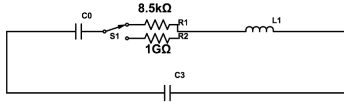
Figure 4. Stimulating Circuit
