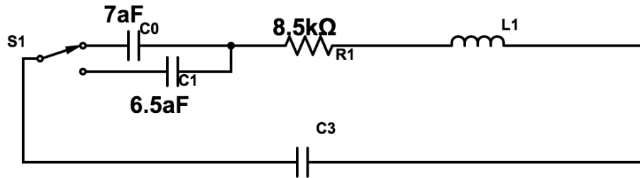
Figure 6. MEMS Resonator Model
