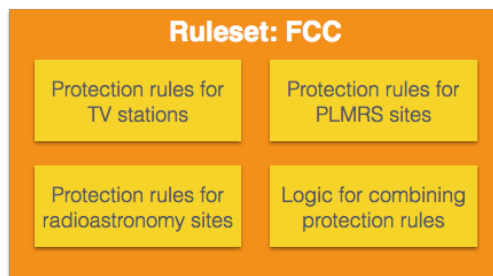
Figure 11.16: Visual representation of a Ruleset object.
