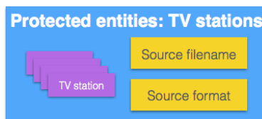
Figure 11.11: Visual representation of a ProtectedEntitiesTvStations object.
