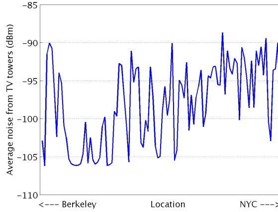
Figure 4.8: Average noise level for secondaries operating in the TV whitespaces along the line shown in Figure 4.6.
