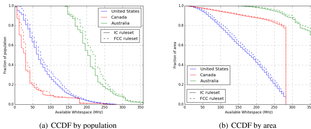
Figure 11.4: Complementary cumulative distribution functions (CCDFs) of available whitespace by population and area in the United States, Canada, and Australia for fixed devices.
