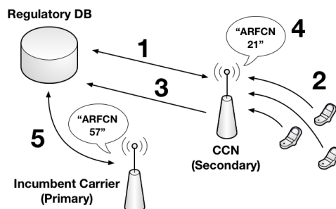
Figure 9.1: Overview of Nomadic GSM. (1) The secondary initially queries a regulatory database for available channels in its area. (2) The secondary gathers measurement reports from its subscribers' phones. (3) Secondaries report spectrum usage (both their own and measured) and service usage (e.g., number of calls and SMS) to a database on a regular basis. (4) Secondaries use measurement report data and guidance from the reg. DB to pick future non-interfering channels to use, and regularly change channels. (5) Optionally, primaries update the regulatory database with their own spectrum usage and query it to obtain reports on what spectrum in use by secondary operators.
