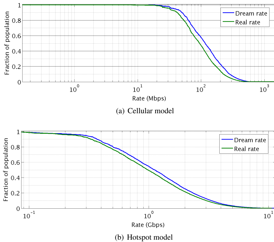
Figure 3.15: CCDFs by population of dream rates and actual rates
