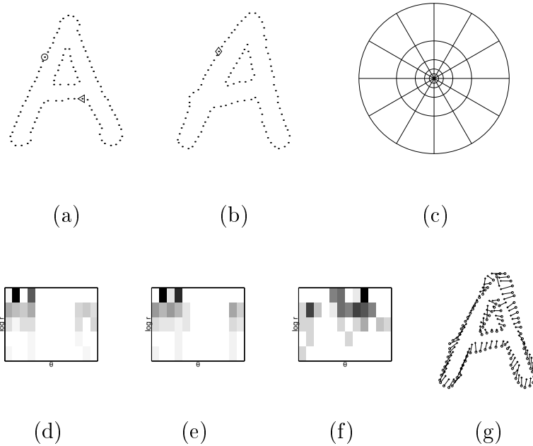
Figure 3. Shape context computation and matching. (a,b) Sampled edge points of two shapes. (c) Diagram of log-polar histogram bins used in computing the shape contexts. We use 5 bins for \log r and 12 bins for \theta . (d-f) Example shape contexts for reference samples marked by \circ , \diamond , \triangleleft in (a,b). Each shape context is a log-polar histogram of the coordinates of the rest of the point set measured using the reference point as the origin. (Dark=large value.) Note the visual similarity of the shape contexts for \circ and \diamond , which were computed for relatively similar points on the two shapes. By contrast, the shape context for \triangleleft is quite different. (g) Correspondences found using bipartite matching, with costs defined by the \chi^2 distance between histograms.
