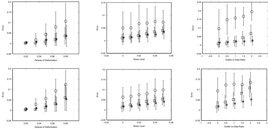
Figure 6. Comparison of our results ( \square ) to Chui and Rangarajan ( * ) and iterated closest point ( \circ ) for the fish and Chinese character, respectively. The error bars indicate the standard deviation of the error over 100 random trials. Here we have used 5 iterations with \lambda_o = 1.0 . In the deformation and noise tests no dummy nodes were added. In the outlier test, dummy nodes were added to the model point set such that the total number of nodes was equal to that of the target. In this case the value of \epsilon_d does not affect the solution.
