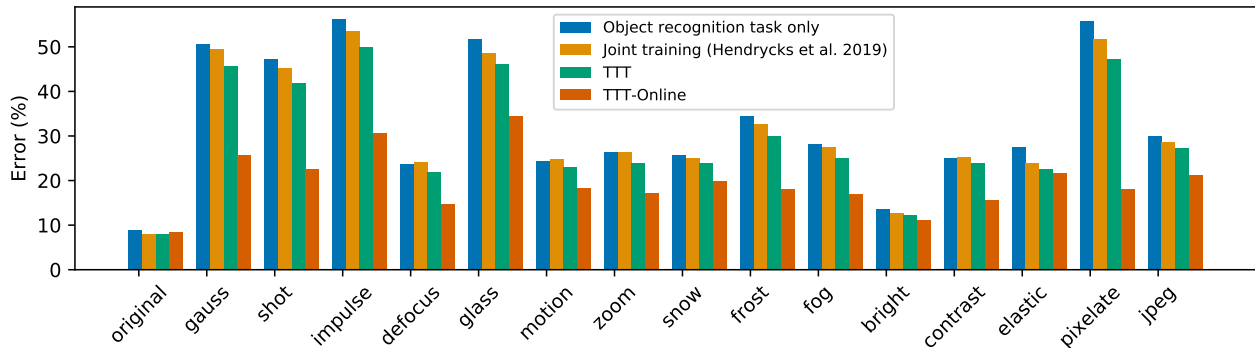
Figure 2.1: Test error (%) on CIFAR-10-C with level 5 corruptions. We compare our approaches, Test-Time Training (TTT) and its online version (TTT-Online), with two baselines: object recognition without self-supervision, and joint training with self-supervision but keeping the model fixed at test time. TTT improves over the baselines and TTT-Online improves even further.
