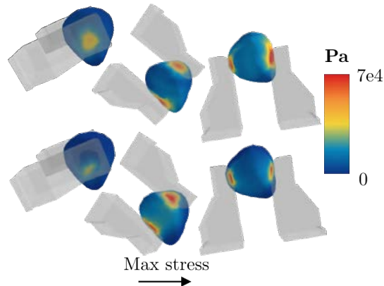
(b) Strawberry, F_g = 6\text{N} , E = 5e4
