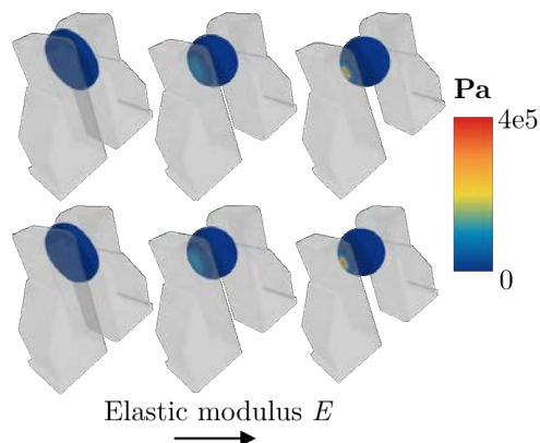
(c) Sphere, F_g = 5\text{N} , E \in [5e5, 1e6, 5e6]
