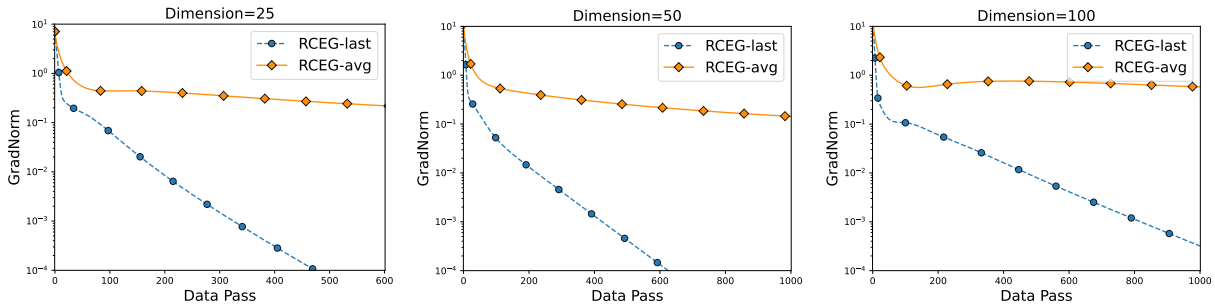
Figure 4.3: Comparison of last iterate (RCEG-last) and time-average iterate (RCEG-avg) for solving the RPCA problem when \alpha = 2.0 . The horizontal axis represents the number of data passes and the vertical axis represents gradient norm.
