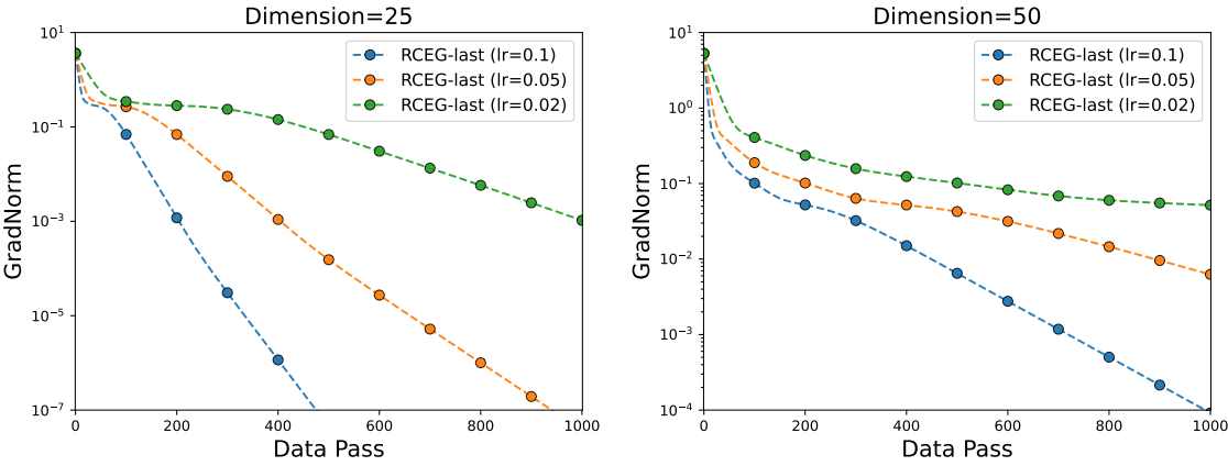
Figure 4.4: Comparison of different step sizes ( \eta \in \{0.1, 0.05, 0.02\} ) for solving the RPCA problem with different dimensions when \alpha = 2.0 . The horizontal axis represents the number of data passes and the vertical axis represents gradient norm.
