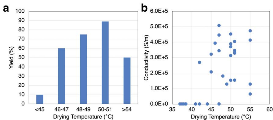
Figure 2.16: a) Yield as a function of drying temperature for 31 printed 30:1:8 Zn:PCL:Anisole traces on PET which were treated with 50% acetic acid solution for 13 minutes. Each bin includes n=4 to n=20 samples. These samples were dried on a hotplate with local heat variation and individual samples' temperatures were measured. b) Conductivity of the traces shown in (a) as a function of drying temperature. Temperatures below 45^{\circ}\text{C} or above 55^{\circ}\text{C} produce mainly non-conductive traces. Within the optimal temperature window, there is not a clear relationship between temperature and conductivity.
