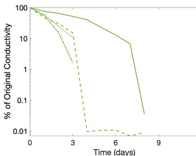
Figure 2.17: PVP-based traces, even when encapsulated with beeswax, lost their conductivity completely within 3-7 days or less.
