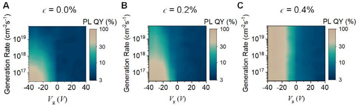
Figure 3.3: PL QY versus G and V_g in WS_2 at different strains. A color plot of PL QY in monolayer WS_2 as a function of gate voltages and generation rate with applied strains.
