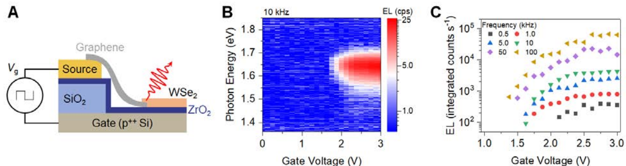
Figure 5.4: Low voltage transient EL from WSe 2 . (A) Cross-sectional schematic, and (B) EL mapping as a function of photon energy and gate voltage. (C) Integrated EL counts showing device turn-on near the gate voltages comparable with bandgap photon energy of monolayer WSe 2 .
