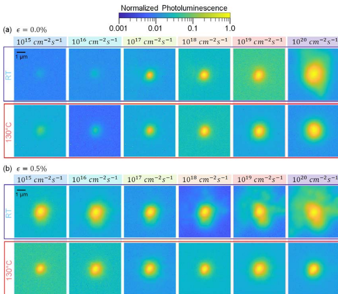
Figure 4.13: Exciton diffusion on heated monolayer (A,B) PL images of counterdoped monolayer WS 2 as a function of generation rate and strain at different substrate temperature. Scale bar is 1 \mu\text{m} . No significant enhancement was observed in the exciton diffusion when the substrate temperature was changed from room temperature to 130^\circ\text{C} .
