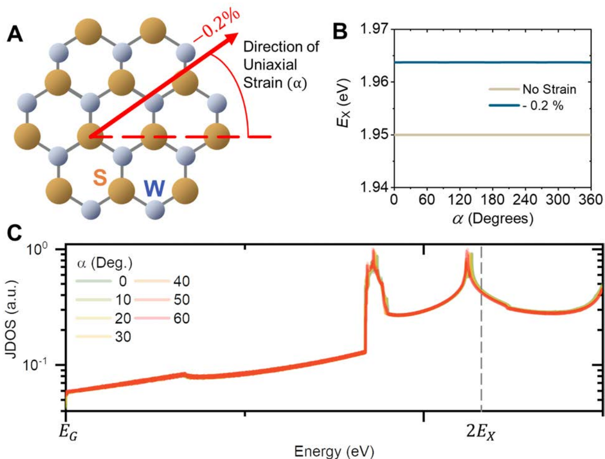
Figure 3.9: Direction independence of EEA suppression. (A) Direction of uniaxial strain (B) Exciton transition energy as a function of strain direction (C) VHS is shifted from twice of exciton transition energy independent of compressive strain direction.
