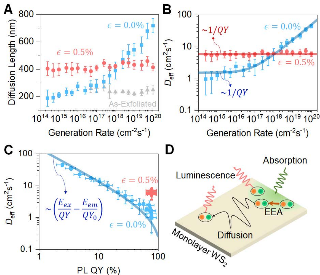
Figure 4.11: Exciton-exciton annihilation enhanced diffusion. (A) Diffusion length of neutral excitons in monolayer WS 2 at different generation rates and strains. (B) Effective diffusion coefficient D_{eff} versus generation rate for monolayer WS 2 with different strains at \epsilon = 0\% , 0.5\% . (C) Inversely proportional relationship between D_{eff} and PL QY, which can be switched by strain. (D) Annihilation of an exciton provides additional kinetic energy to another nearby exciton to traverse further and then emit light, resulting in a large diffusion pattern.
