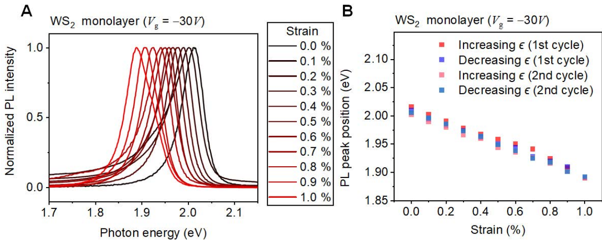
Figure 3.4: PL peak position shift of monolayer WS_2 . (A) Normalized PL intensity of monolayer WS_2 at V_g = -30 V as a function of applied strains. (B) PL peak position during multiple bending and release cycles.
