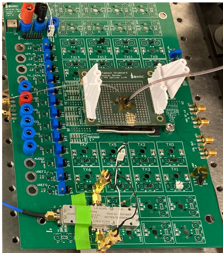
Figure 5.10: Host board in test setup for MRI system. Chip board in zero insertion force socket with fiber attach and fiber stress relief posts shown in center of board.
