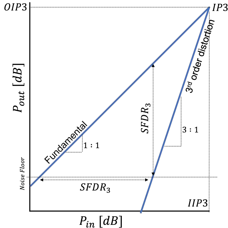
Figure 4.22: Output fundamental and third order power versus input power. The noise floor, independent of input power, plotted as a horizontal line. SFDR 3 represents the maximum dynamic range achievable, bounded by the noise floor on the low end, and the power at which the third order intermodulation spur rises above the noise floor on the high end.
