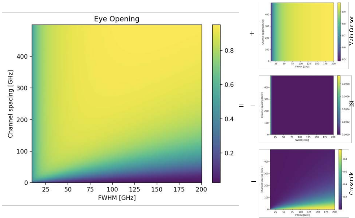
Figure 3.12: Eye opening versus FWHM design bandwidth and channel spacing for a single drop ring filter. The relevant ring parameters are: Q_0 = 100000 , \text{FSR} = 17 \text{ nm} , and \lambda_0 = 1280 \text{ nm} . The bitrate is 10Gbps. The subplots on the right show the contributions to eye opening from the main cursor, ISI, and crosstalk (from top to bottom).
