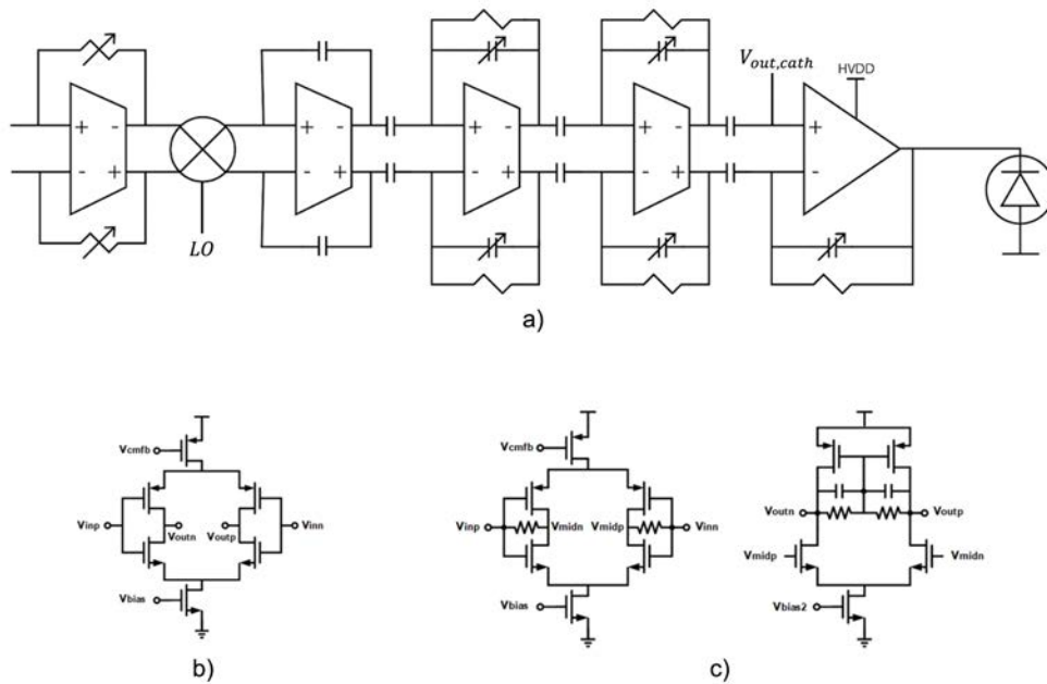
Figure 5.4: Architecture of the MRI receiver / transmit driver for the microring modulator. a) Architecture of the gain chain, including 1 st stage, bypass-able mixer, 2 nd gain stage, two VGA stages, and output driver stage. b) Circuit details for 1 st stage amplifier. c) Circuit details for 2 nd stage amplifier.
