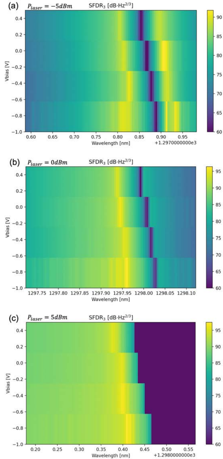
Figure 4.23: (a) SFDR 3 versus electrical and optical bias points, for P_{laser} = -5 dBm. (b) SFDR 3 versus electrical and optical bias points, for P_{laser} = 0 dBm. (c) SFDR 3 versus electrical and optical bias points, for P_{laser} = 5 dBm.
