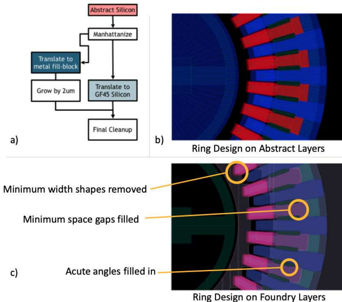
Figure 2.4: a) Sample Dataprep routine, showing the operations performed on shapes on the ‘silicon’ designer layer. In this example process, the silicon shapes are Manhattanized (de-angled) to a user specified grid. In parallel, a 2\mu\text{m} larger fill exclude is generated around the silicon geometry. Finally, these shapes are mapped onto the appropriate foundry layers. b) Sample of a ring modulator in GF45RFSOI, showing the ‘abstract’ designer layers before Dataprep . c) Sample of a ring modulator in GF45RFSOI, showing the foundry layers after Dataprep . Callouts indicate several types of DRC violations that are resolved in the Dataprep process.
