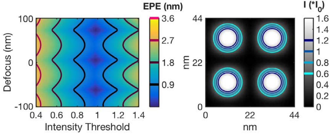
Figure 3.16: Left: EPE_{max} process window for p_{wf} = 22\text{nm} contacts, 0.55 NA, N_{etch} = 26 bilayers. Right: Aerial image at best focus, contours at exposure thresholds.
