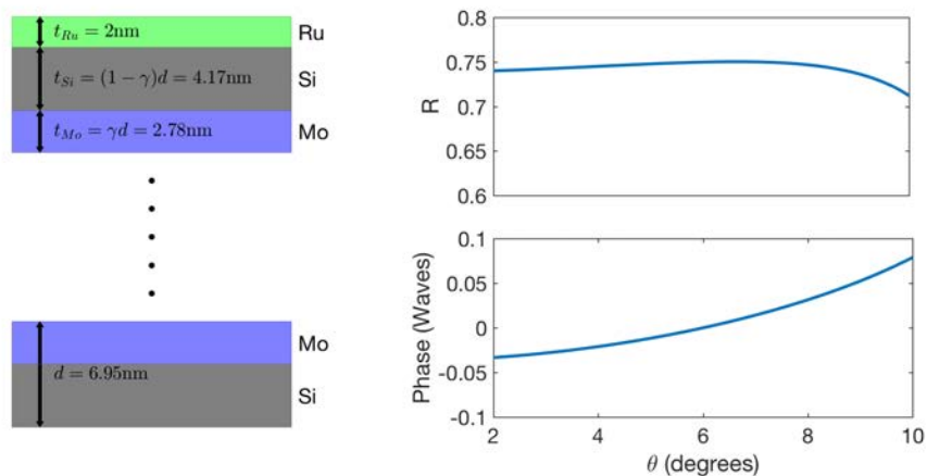
Figure 3.5: Left: multilayer stack design. Right: reflected intensity and phase vs angle. n and k values drawn from CXRO database for \lambda = 13.5\text{nm} . Values used: Si: n = 0.99900154 , k = 0.0018265 ; Mo: n = 0.923791 , k = 0.0064358 ; Ru: n = 0.8864 , k = 0.017066 .
