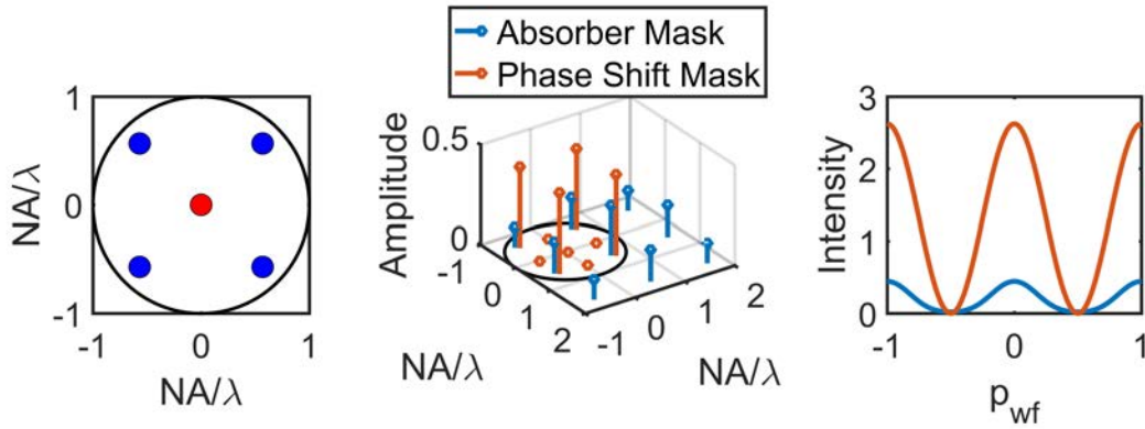
Figure 3.4: Left: Quadrupole illumination for absorber mask (blue) and conventional illumination for phase-shift mask (red). Center: Pupil plane plot of one illumination pole for each mask. Right: Aerial image cross-sections from each mask.
