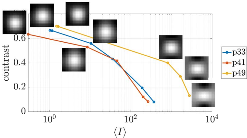
Figure 3.31: aPSM optimization for 3 features, trading off contrast and optical efficiency. Each point represents the optimal solution at one of the 10 \alpha values, after 6 generations of optimization. Inset images display representative examples of the image quality.
