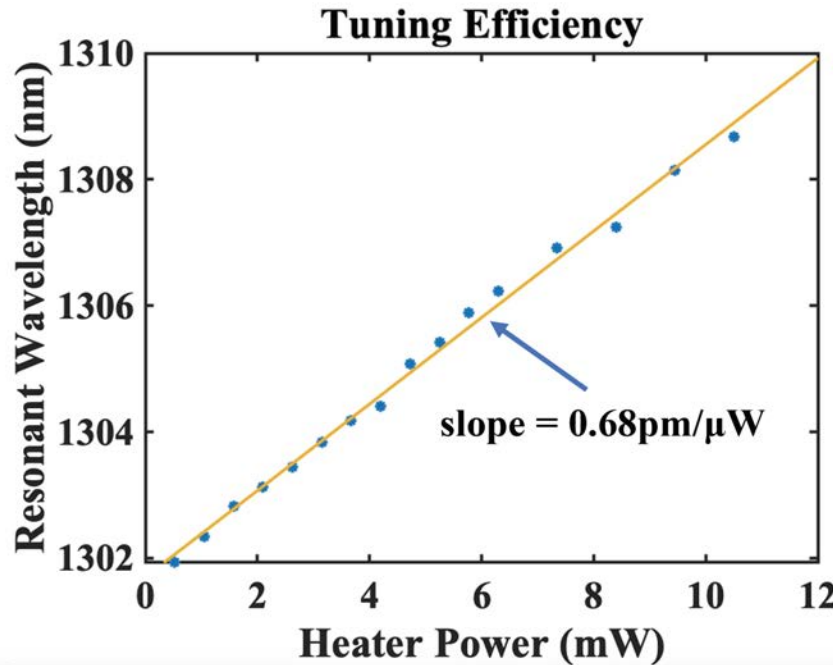
Figure 5.7: Tuning efficiency of the embedded ring heater extracted by sweeping the PDM driver code.
