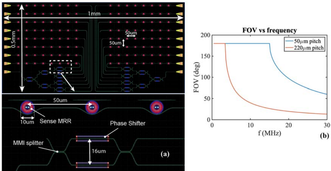
Figure 7.1: (a) Compact BPG generated layout with 50\mu\text{m} MRR pitch, corresponding to \frac{\lambda}{2} of 15MHz ultrasonic signals and a record low sensing element area of 0.0025\text{mm}^2 , (b) Field-of-view vs ultrasound frequency.
