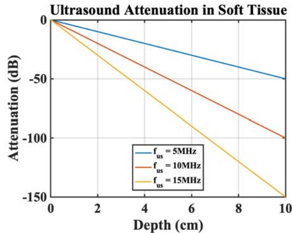
Figure 4.2: Attenuation of ultrasound amplitude in tissue over distance for various excitation ultrasound frequencies.
