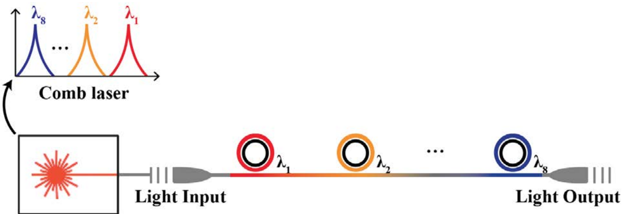
Figure 2.4: Towards a 2-D optical MRR-based ultrasound receiver: A ring row consisting of multiple MRRs coupled onto the same silicon waveguide and interrogated by a comb laser input in a WDM fashion. Arraying multiple such rows in parallel, can form a dense 2-D matrix.
