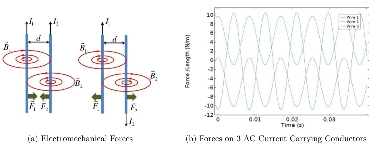
Figure 3.1: Forces on 3 phase AC conductors
