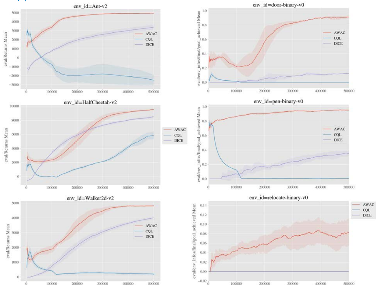
Figure 74: Comparison of our method (AWAC) with CQL and AlgaeDICE. CQL and AWAC perform similarly offline, but CQL does not improve when fine-tuning online. AlgaeDICE does not perform well for offline pretraining.
