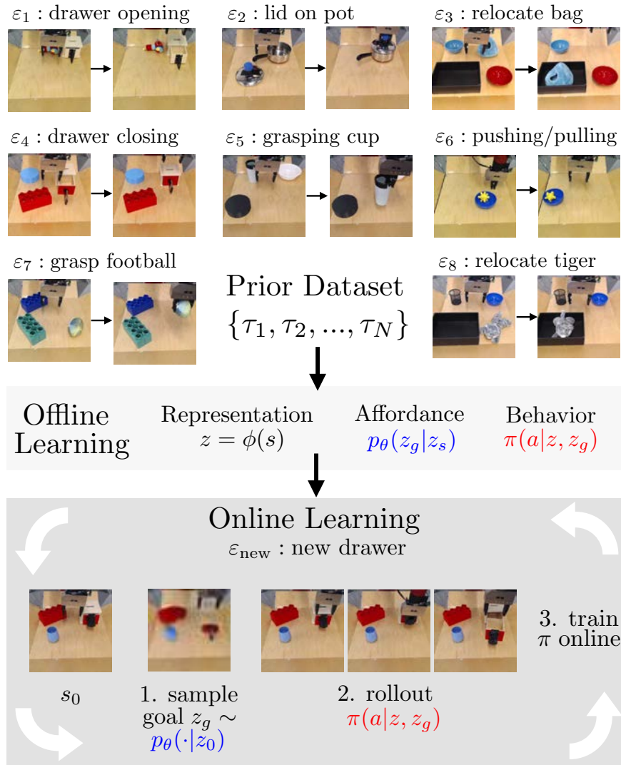
Figure 49: We propose a system for efficient self-supervised robot learning in an unseen environment \mathcal{E}_{\text{new}} by utilizing prior data \mathcal{D} of trajectories from related similar environments \mathcal{E}_i \sim p(\mathcal{E}) . Tasks are specified via a target goal image. From prior data, we learn an encoder \mathbf{z} = \phi(\mathbf{s}) of images (representation) for compressing observations and self-generating rewards, a model of what tasks might be tested in the new environment (affordance), and goal-conditioned policy to accomplish a given task (behavior). While this provides reasonable performance in some test environments, perfecting the policy in test environments may require additional interaction in the test environment. Dropped in a test environment \mathcal{E}_{\text{new}} without a given goal, we run RL online in order to practice potential tasks, with goals sampled from the affordance model. Online behavior learning allows us to improve the policy \pi for \mathcal{E}_{\text{new}} even when it contains new and unseen objects.
