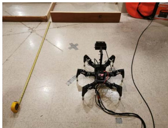
Figure 2.20: Test 3: hexapod starts at 1m from 20cm joist. The resulting grid map images and line detections for this experiment are shown in Appendix C. Demo video .
