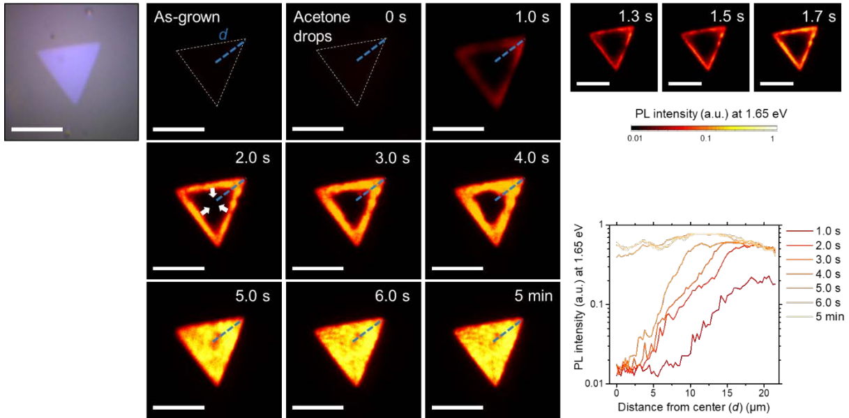
Fig. S1. In-situ PL imaging of as-grown WSe 2 monolayer during the SEMD process. The scale bars are 30 \mu\text{m} for all images. Note that the PL images were taken with 1.65 eV bandpass filter to block the emission from as-grown WSe 2 monolayer. The bottom right plot shows the PL intensity profile of the WSe 2 monolayer at 1.65 eV during the SEMD process.
