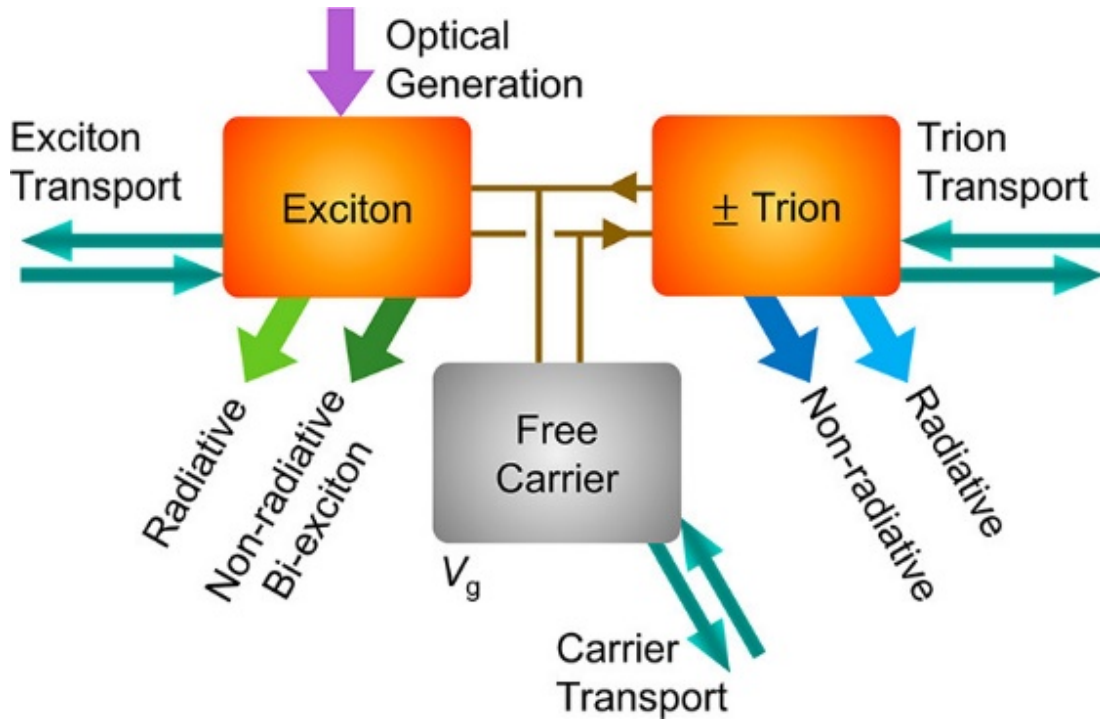
Fig. 2. In a differential area, exciton concentration increases by 1. generation upon absorption of a photon, 2. exciton transport into the area resulting from concentration or potential gradients, and 3. ionization of trions. Exciton concentration decreases by 1. trion formation, 2. radiative recombination and 3. bi-excitonic recombination. Similar generation and recombination processes occur for trions. The ratio of excitons and trions are controlled by the background carrier concentration, which also can drift and diffuse.
