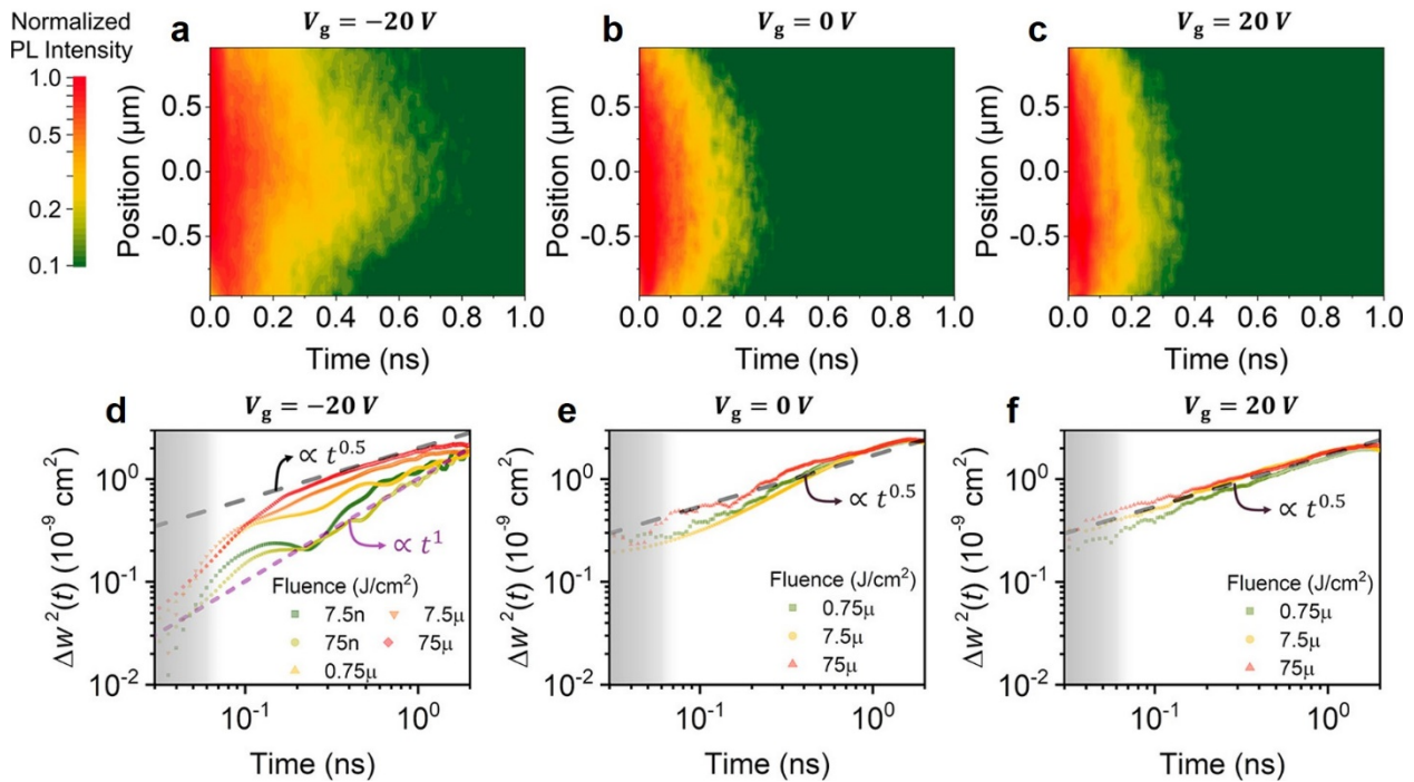
Fig. 5. a, b, c , Map of emission intensity as it evolves in space and time at V_g = -20 \text{ V} , 0 \text{ V} , and 20 \text{ V} , respectively at a pump fluence of 75 \mu\text{Jcm}^{-2} . d, e, f , Time evolution of differential squared width for various pump fluence at V_g = -20 \text{ V} , 0 \text{ V} and 20 \text{ V} , respectively. The instrument response function (IRF) has a FWHM of \sim 50 \text{ ps} , which is shown as a shaded region.
