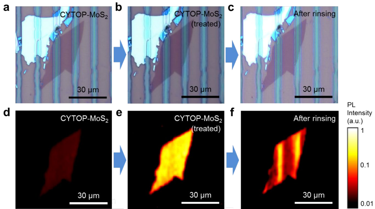
Fig. 5. a to c Optical micrographs, and d to f corresponding photoluminescence images of an as-prepared CYTOP-patterned MoS 2 monolayer, after treatment by TFSI, and after rinsing with water for 15 seconds; PL images are plotted on a common logarithmic scale.
