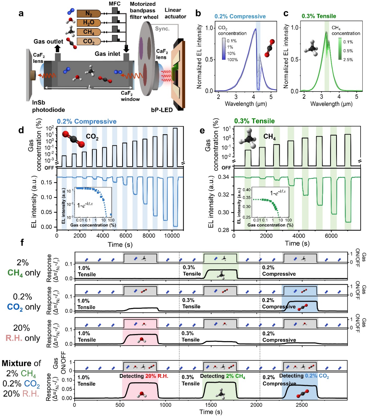
Fig. 4. a, Schematic diagram of the NDIR gas sensing system using a strain-tunable bP-LED. b, c,
