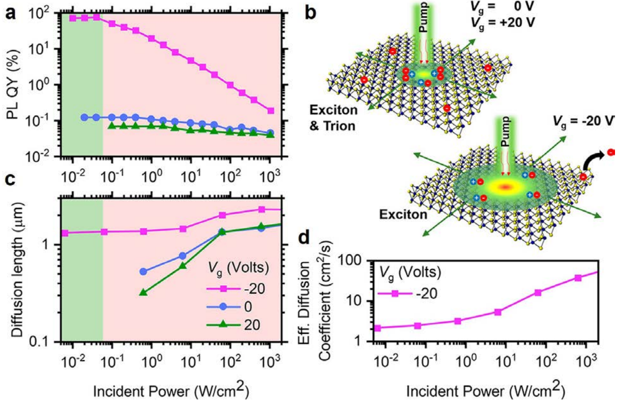
Fig. 4. a , Pump-power dependence of the PL QY for electrostatically-doped MoS 2 . b , Exciton and trion diffusion in MoS 2 . c , Diffusion length of a MoS 2 device under V_g = 0\text{V} , V_g = -20\text{V} and V_g = 20\text{V} . d , Effective diffusion coefficient for neutral excitons in MoS 2 at different pump power.
