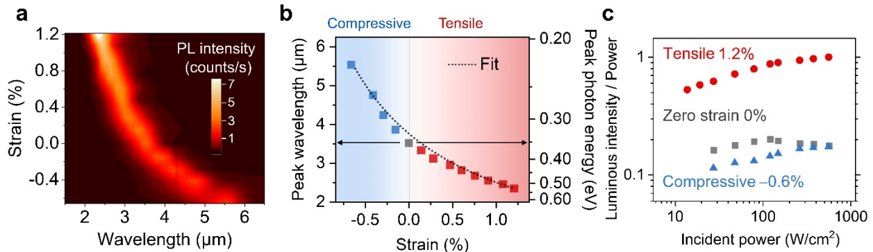
Fig. 2. a , PL spectra of bP as a function of strain along the ZZ ( y ) direction. b , Strain-dependent PL spectral peak shift in bP. The fit indicates that the peak modulation rate is 1.70 μm wavelength shift per percent of strain, covering from 5.5 to 2.3 μm. Laser-induced thermal effects on strain are precluded by using low excitation power, where the PL spectral peak is constant with increasing laser power density (Fig. S2b). c , Integrated PL intensity normalized by incident power as a function of power density for bP under different strain conditions. Note that bP thickness is 20 nm in the above measurements. We also demonstrated reversible and repeatable bandgap tuning, which indicates that there is no mechanical slip between bP and the substrate over multiple cycles (Fig. S2e).
