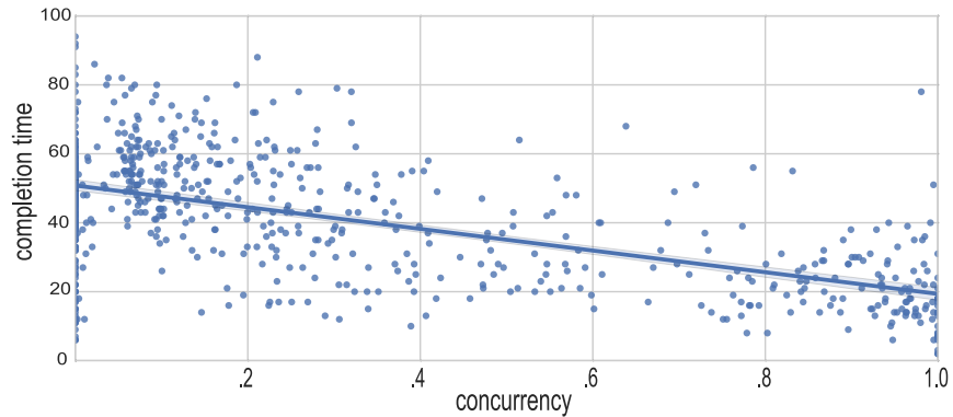
Figure 2.5: Completion time correlated with level of concurrency. A negative correlation suggests that concurrent interactions may help alleviate the effect of latency.
