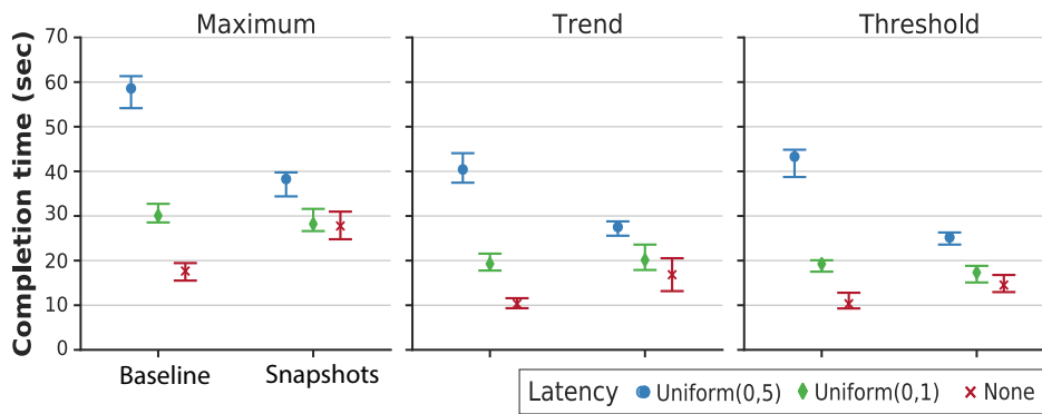
Figure 2.6: Each chart of the plot visualizes median task completion time with 95% CI (y-axis).
