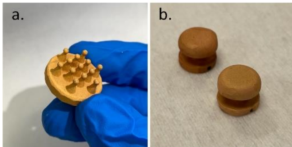
Figure 3: 3D printed and electroless plated electrodes. (a) Pin style electrodes optimized for comfortable EEG recording. (b) More general button style electrodes suitable for hairless site recordings such as EMG or ECG.
