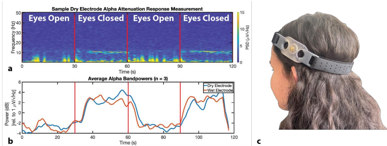
Figure 10: Electroencephalography. (a) Sample Time-frequency spectrogram of a single dry electrode alpha attenuation response. (b) Averaged ( n=3 ) alpha (8-12 Hz) band power of alpha modulation recorded across a subject's scalp for both dry pin and wet gold cup electrode measurements. Alpha power increased by a factor of 5x in the eyes-closed state for both dry and wet measurements. (c) Alpha attenuation response measurement setup. Two dry electrodes were placed on either side of the head.
