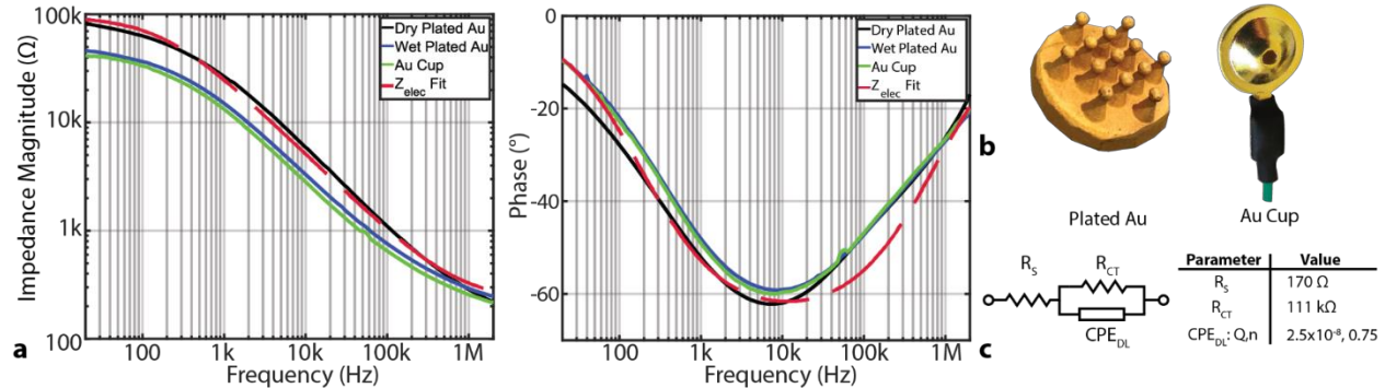
Figure 6: Electrode-skin interface (ESI) characterization of the gold-plated pin electrodes vs clinical gold cup electrodes. (a) Average ( n = 5 ) magnitude and phase of gold-plated pin electrodes on scalp with and without electrolyte gel alongside gold cup electrodes. An electrode model with a constant phase element (CPE) model, Z_{elec} , was fitted to the dry gold-plated pin electrodes. (b) 3D-printed, gold-plated, dry EEG electrode (left) and clinical gold cup electrode (right). (c) CPE model with fitted parameters for spread resistance R_s , charge transfer resistance R_{ct} , and CPE double layer, C_{dl} .
