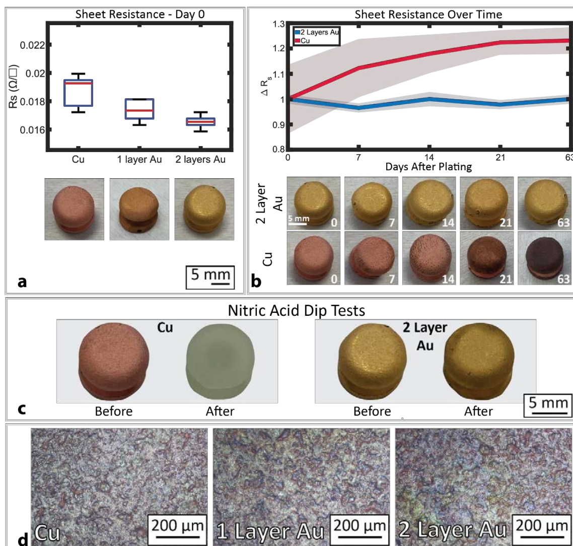
Figure 5: Electrical and physical characterizations of Au plated surfaces. (a) Box plot of absolute sheet resistance immediately after plating. In each box, the red mark indicates the median while the top and bottom of the boxes represent the 25th and 75th percentiles, respectively. The whiskers extend to the most extreme data points. (b) Sheet resistance over time normalized to day 0. Photos of the copper and copper + two layers of gold samples across the 9-week longevity study. (c) Before and after photographs of acid dip test. The copper sample was etched bare, while the double layered gold sample showed no effect. (d) Light microscopy images of plated surfaces showcasing the roughness resulting from sandblasting.
