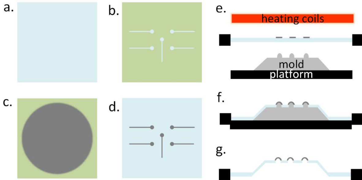
Figure 1: Printing and vacuum forming process flow. (a) Polycarbonate substrate. (b) Substrate is masked with PET tape and design is laser cut and peeled off. (c) Silver ink is deposited via airbrush. (d) Tape is peeled off. (e) Substrate is then clamped into vacuum former where it is heated from above. (f) After substrate is pliable and heating coils are pulled back, the platform with the mold is raised and vacuum is drawn. (g) The substrate quickly cools and retains its shape when the mold is removed.
