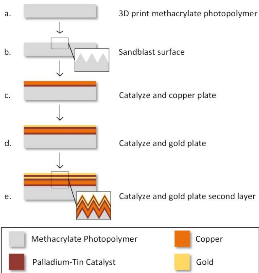
Figure 4: Fabrication process flow. (a) Design is 3D printed. (b) Sample is sandblasted, cleaned, and exposed to surfactant. (c) Catalyst, and copper plating solutions create a thick copper base. (d) Samples are submerged in surfactant, catalyst, and gold plating solutions. (e) The gold plating steps are repeated one once more for an improved diffusion barrier.
