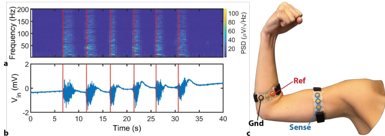
Figure 9: Electromyography. (a) Spectrogram and (b) time-domain of EMG measurements taken with two electrode bands (c) placed along a single subject's arm. The subject was cued to flex their bicep every 5 seconds. Characteristic broad spectrum muscle activity ( \sim 0 - 200 Hz) was observed when the user was cued to flex.
