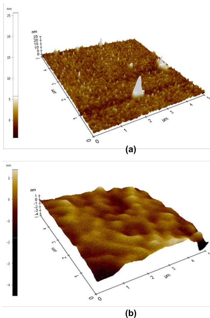
Figure 5.9: surface roughness of WO 3 /Ag/WO 3 and ITO anodes. 3D AFM height images of (a) WO 3 /Ag/WO 3 and (b) ITO on PEN acquired by non-contact mode Park Systems Atomic Force Microscope. The WO 3 /Ag/WO 3 film has a 1.5 nm RMS surface roughness and 25.4 nm peak roughness. The ITO film has a .5 nm RMS surface roughness and 1.4 nm peak roughness.
