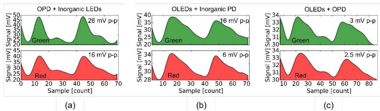
Figure 4.14: Photoplethysmograms (PPGs) acquired using combinations of inorganic and organic LEDs and photodiodes (PDs). (a) PPG signal acquired using inorganic red and green LEDs and an OPD. Green and red PPG signal amplitudes of 26 mV_{p-p} and 16 mV_{p-p} were obtained, respectively. (b) PPG Signal acquired using OLEDs and silicon PD - reduced irradiance of the OLEDs bring down signal magnitude to 16 mV_{p-p} and 6 mV_{p-p} upon green and red excitation. (c) PPG signal acquired using OLEDs and OPD; although signal magnitudes are reduced to 3 mV_{p-p} and 2.5 mV_{p-p} , the signal is sufficient for resolving the PPG waveform and provide the light absorption ratio ( R_{os} ) information for blood oxygenation calculation.
