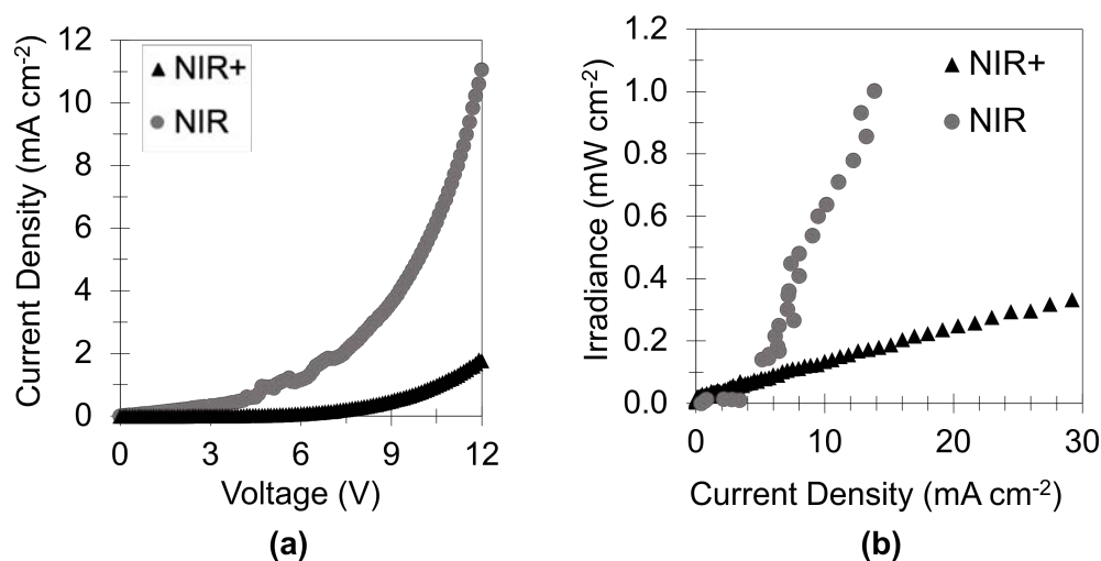
Figure 7.5: NIR and NIR+ OLED device performance. Looking at the NIR and NIR+ OLED’s stand-alone device performance characteristics, the NIR+ OLED has inferior diode characteristics with (a) lower current densities as a function of voltage and (b) irradiance as a function of current density. While the NIR OLED’s maximum irradiance was 1 \text{ mWcm}^{-2} , the NIR+ OLED’s irradiance only reached .33 \text{ mWcm}^{-2} . This underscores the importance and impact of wavelength in an optical biomedical device: despite poor device characteristics, the NIR+ OLED produced a better PPG signal (as shown in Figure 7.3).
