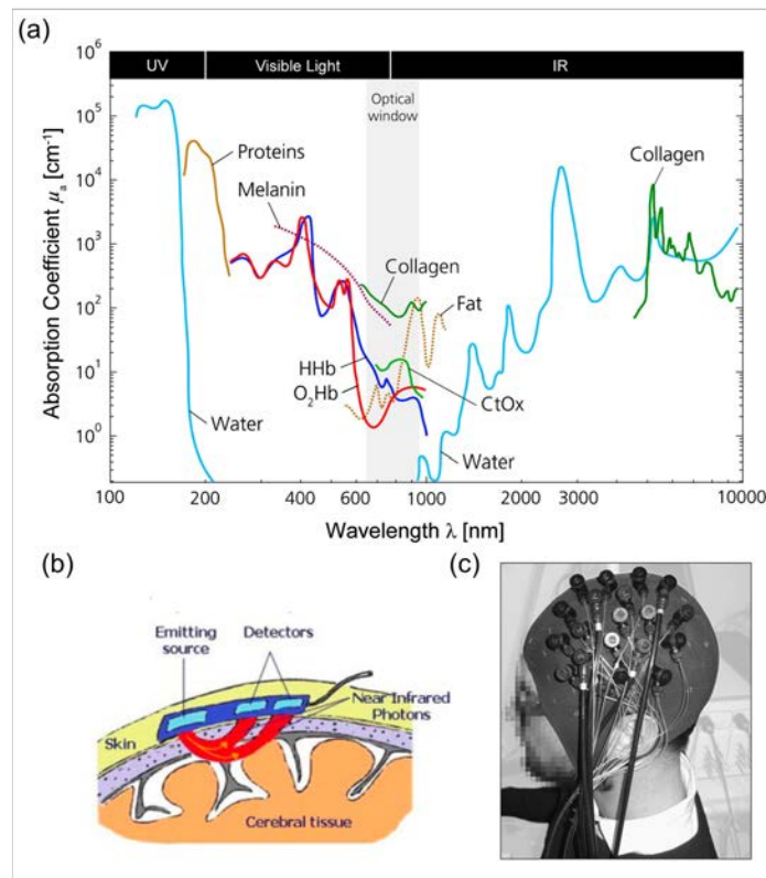
Figure 2.4: Near infrared spectroscopy (NIRS) . (a) The absorption coefficient of chromophores in biological tissue (water, protein, melanin, collagen, fat, cytochrome oxidase, and oxygenated and deoxygenated hemoglobin) as a function of wavelength. The NIR optical window between 650-950 nm (shaded in grey) is where light has the deepest penetration depth in biological tissue and hemoglobin accounts for the majority of light absorption because hemoglobin is present in higher concentrations than the other chromophores with larger absorption coefficients [37]. (b) Schematic of the path of photons for an NIRS device worn on the skull [39]. (c) An experimental cranial fNIRS probe with optical fibers carrying optical signals. [37].
