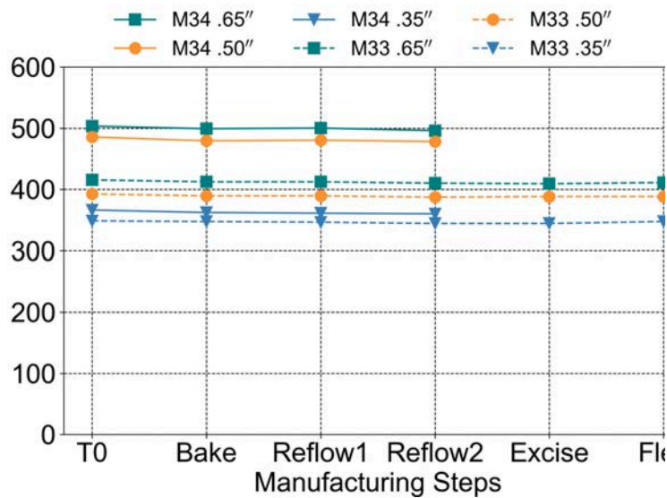
Figure 6.19. The TV array resistance after various manufacturing steps, thermal cycling, and flexing. T0 was immediately after the manufacturing build; bake followed solder mask cure at 150 °C for 1 hr; reflows 1 and 2 were performed at a simulated solder reflow at 205 °C, and excise was done to check for a response after the parts were cut from the substrate tensioned on a frame. Flex step was done at 1000 bend cycles on a 2 mandrel. Results for 6 arrays are shown, where the length of the arrays was varied from 0.35" to 0.65".
