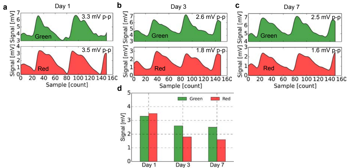
Figure 3.8. Stability of the all-organic optoelectronic sensor. (a,b,c) Recorded signal intensities on day 1, 3, and 7 respectively after fabrication of the sensor. (d) Bar chart showing the degradation in signal intensity over seven day time period. Decline in performance is mainly due to encapsulation failure of the organic optoelectronics.
