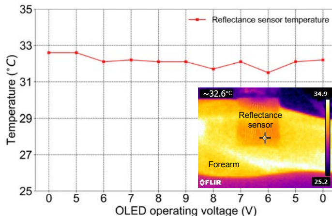
Figure 5.15. Reflectance sensor temperatures on the forearm. The sensor OLEDs are operated using drive voltages from 0 to 9V, and the temperature of the reflectance sensor is recorded. The temperature remains within 32 \pm 0.5^\circ\text{C} under the different drive conditions. The inset shows the thermal photo of the measurement setup. A thermal camera is used to record the sensor temperatures.
