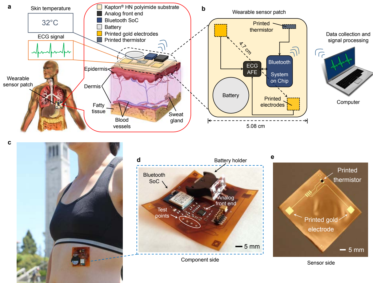
Figure 6.1. Proposed overview and system design of the wearable sensor patch (WSP) enabled by flexible hybrid electronics. (a) Schematic of the sensor patch placed on a subject's lower left rib cage. Skin temperature is read using a stencil-printed thermistor while the electrocardiography (ECG) signal is acquired using inkjet-printed gold electrodes. The electrodes and the thermistor are interfaced to silicon-based ICs for data acquisition, processing, and transmission. (b) System design of the sensor patch. The ECG signal is obtained using an analog front end (AFE). The data is then processed and transmitted using a Bluetooth System on Chip (SoC) to a host computer. The thermistor data is read using a voltage divider network, where the voltage drop across the thermistor is sensed using an analog to digital converter (ADC) of the SoC. After data transmission, both ECG and thermistor data are displayed on a host computer. (c) Photograph of the WSP mounted on a person's lower left rib cage. The sensor side faces down towards the skin, and the component side faces up. (d) Photograph of the component side of the patch. The battery holder, the Bluetooth SoC, AFE, and the test points are shown. (e) Photograph of the sensor side of the patch (before component assembly). The printed gold ECG electrodes and the thermistor are shown.
