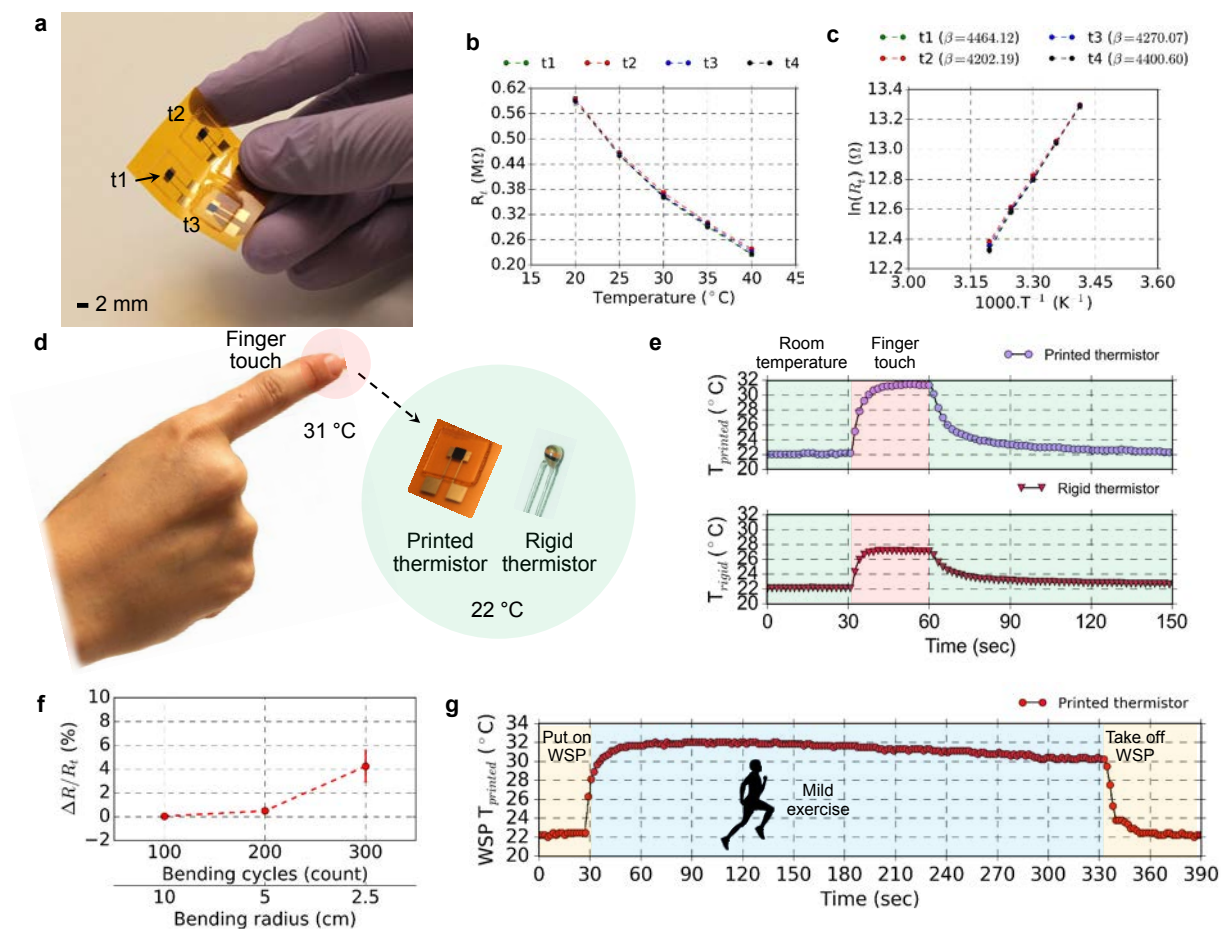
Figure 6.5. Characterization and dynamic testing of the stencil-printed thermistors. (a) Photograph of stencil-printed thermistors composed of NiO nanoparticles and PSBR binder on Kapton ® PI substrate. The four thermistors are labeled t1, t2, t3, and t4. (b) Resistance vs. temperature plot for the thermistors. (c) \beta plot of the printed thermistors. (d) Characterization of the dynamic response of the printed thermistor. The printed thermistor and a commercial rigid thermistor are used to study the dynamic response. Both thermistors are touched with an index finger to record the change in temperature (22 to 31 ^{\circ} C). (e) The top panel shows the temperature read by the flexible thermistor and the bottom panel shows the temperature read by the rigid device. At normal condition (green), both thermistors show 22 ^{\circ} C, after touching the thermistors (red), the resistance drops due to the rise in temperature. As a result, the printed thermistor show 31 ^{\circ} C, and the rigid thermistor show 27 ^{\circ} C. (f) Durability testing of the printed thermistors. Bending radii of 10, 5, and 2.5 cm are used, and the thermistors are subjected to 100 bending cycles at every bending radius. The room temperature resistance of the thermistors roughly changed by 0, 0.5, and 4%, respectively (the error bars represent data collected from 8 devices). (g) Real-time temperature monitoring using the thermistor. The thermistor accurately measured skin temperature of 30 - 32 ^{\circ} C during the exercise (blue overlay).
