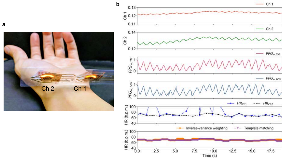
Figure 4.11. HR detection using TM and IVW algorithms from the printed multi-channel PPG sensor. (a) The printed sensor is placed on the underside of the wrist. (b) Ch 1 and Ch 2 are PPG data collected from the ulnar and the radial arteries, respectively. PPG_{w, TM} and PPG_{w, IVW} are the weighed PPG signals generated by TM and IVW algorithms. HR_{Ch1} and HR_{Ch2} are calculated HR by using Ch 1 and Ch 2 PPG data. The bottom panel shows calculated HR by TM and IVW algorithms.
