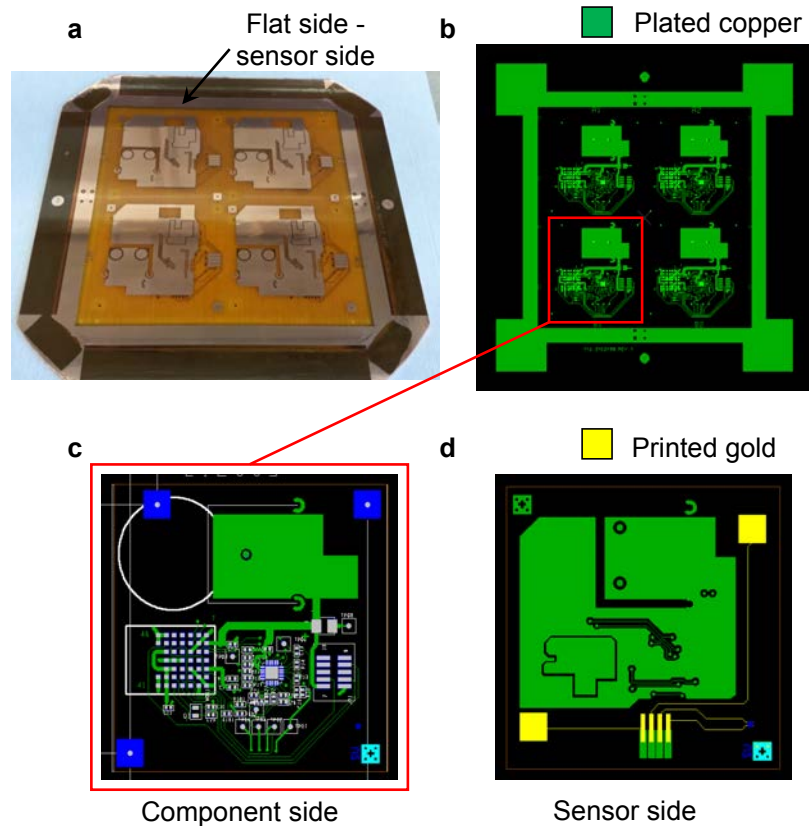
Figure 6.8. Fabrication frame and layout of the WSP. (a) A Kapton ® PI substrate is mounted on a 1.27 mm thick frame. Each frame contains four WSPs. The flat side of the frame where sensors are printed, is displayed. (b) The layout of the full panel consisting of four WSPs. Green patterns represent the plated copper. (c) The layout of the component side. (d) The layout of the sensor side: green represents plated copper while yellow represents the printed gold. Alignment marks are visible, which are used to align the gold layer to the copper layer.
