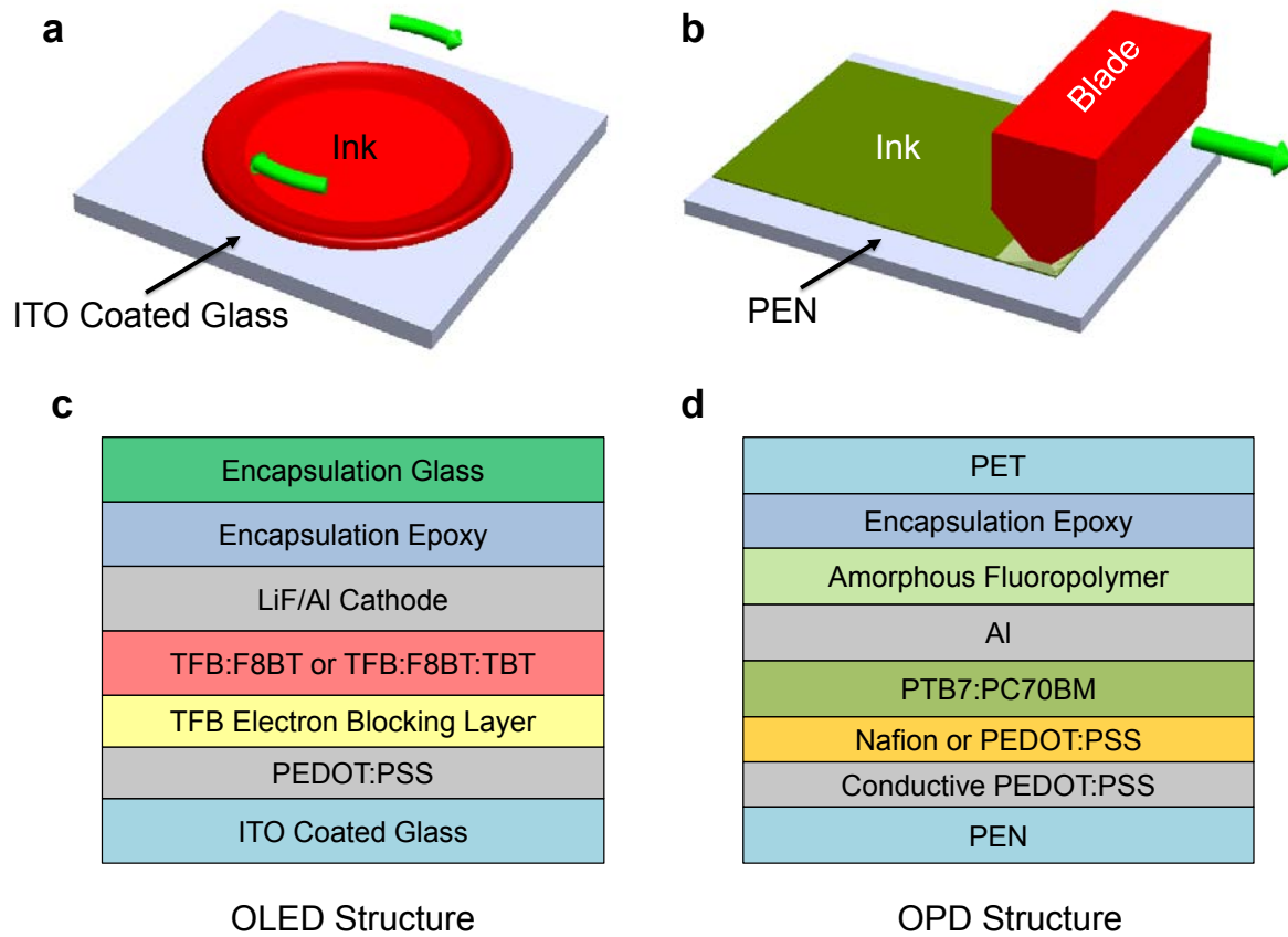
Figure 3.3. OLED and OPD fabrication and physical device structures. (a) The OLEDs are fabricated on a glass substrate using spin coating. (b) The OPDs are fabricated using blade coating on a PEN substrate. (c,d) The physical structures of the OLEDs and OPDs , respectively.
