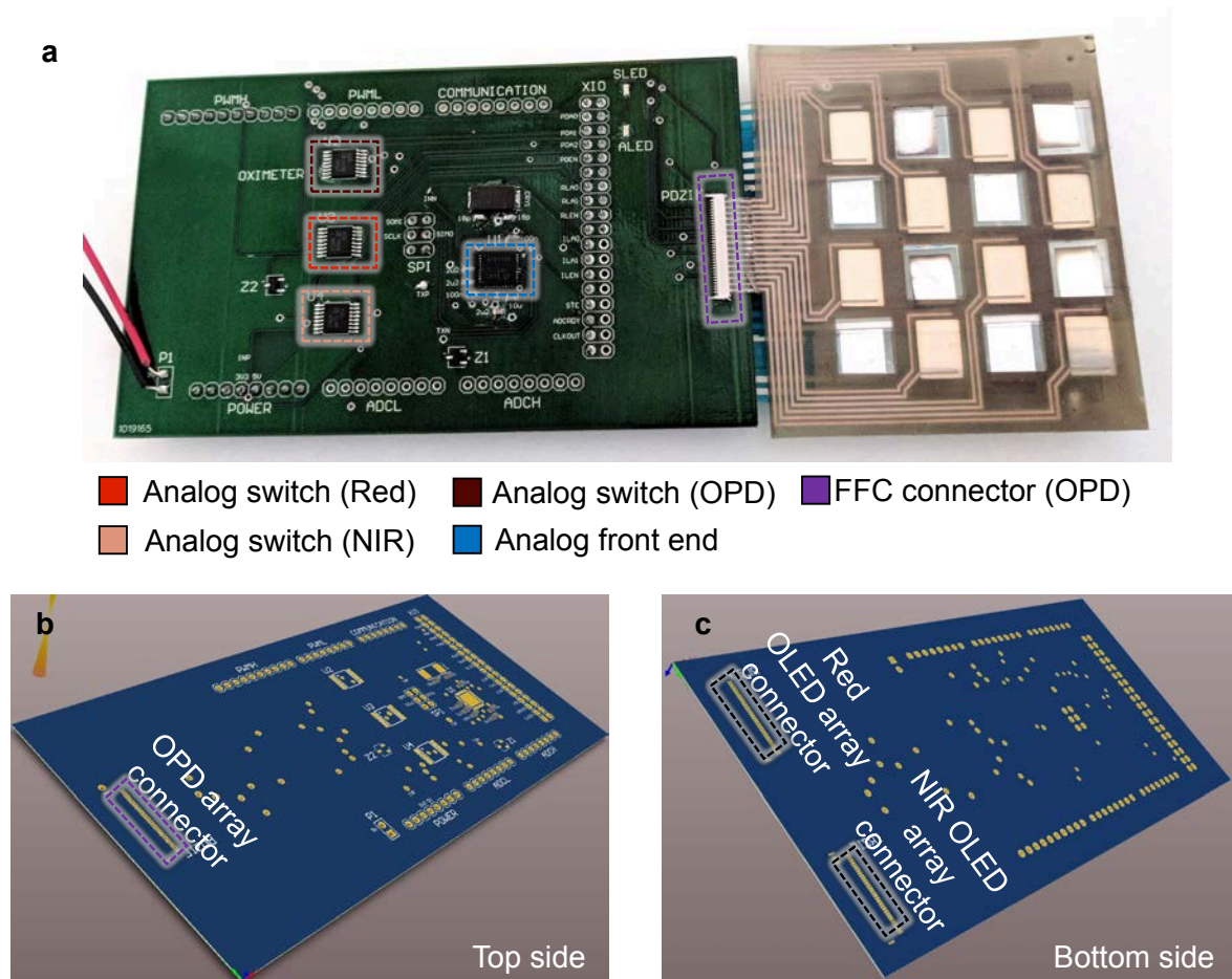
Figure 5.12. Control electronics and connections of the oximeter system. (a) The red and NIR OLED arrays and the OPD array are connected to the control electronics using FFC connectors. These connections then go through three analog switches to the analog front end (AFE 4490). The AFE connects to an Arduino Due microcontroller over Serial Peripheral Interface (SPI) bus, which provides software control of the oximeter array. (b) The top side of the control board, which shows the OPD array connector. (c) The bottom side of the control board, which shows the red and NIR OLED array connectors.
