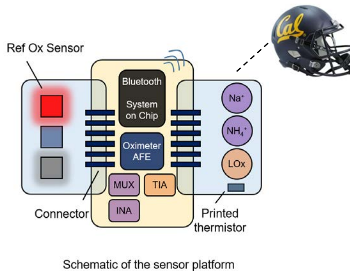
Figure 7.2. An integrated flexible and wearable multi-sensor platform. Both vital signs and analytes in bodily fluids are used to provide an overall snapshot of a person's physiological state.
