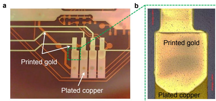
Figure 6.15. Micrographs of the gold/copper interface. (a) Gold ink spreading on copper pads. Copper pads are more hydrophilic than Kapton ® PI surface, as a result, ink spreads on the pads. (b) Zoomed view of the gold/copper interface. Gold ink spread on the surface of copper, and gets pinned at the edges of the pad.
