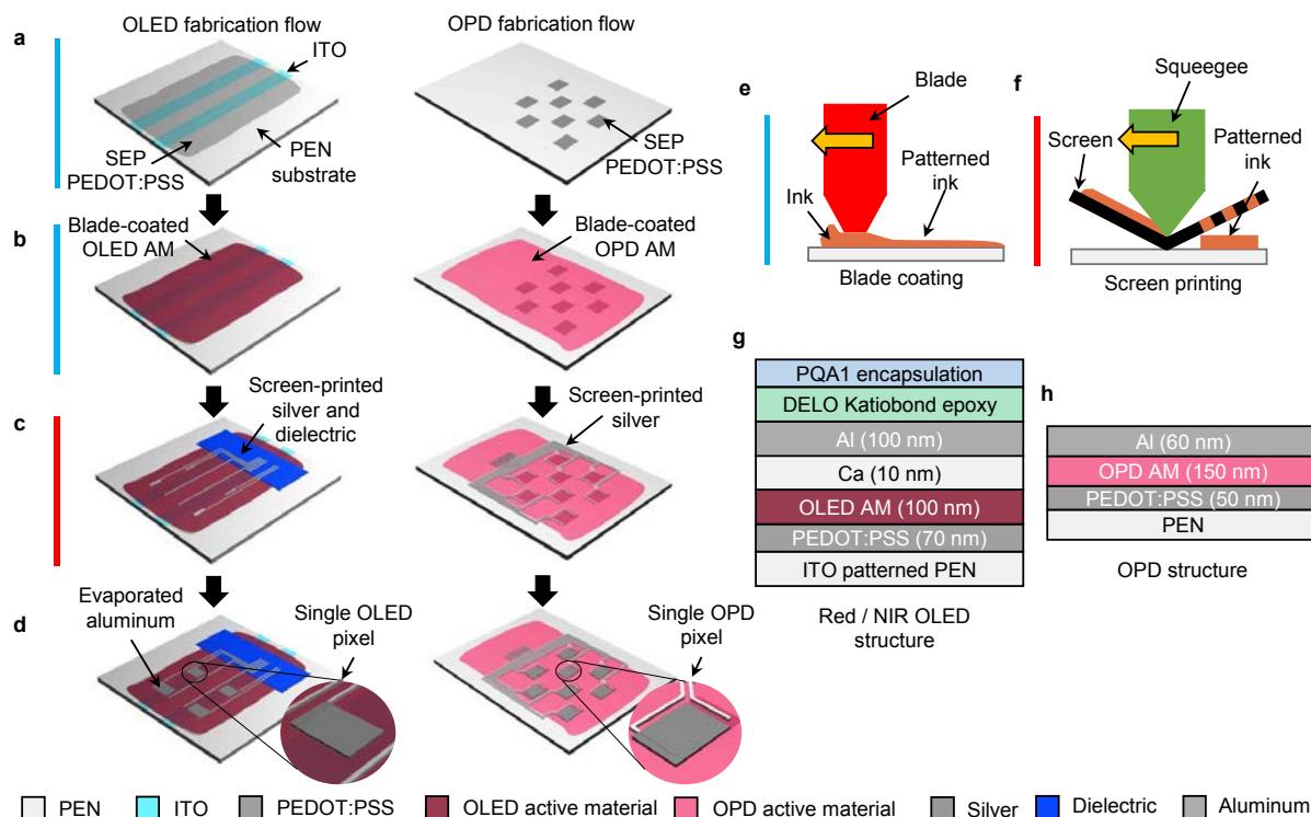
Figure 5.8. Fabrication flow of the OLED and OPD arrays for the ROA . (a-d) The OLED and OPD array fabrication steps are shown side by side. For the OLED array, only one color consisting of four pixels is shown for simplicity - the same fabrication steps are used for red and NIR OLEDs . For the OPD array, the complete array consists of 8 pixels. (a) PEDOT:PSS is blade-coated using surface energy patterning (SEP) on ITO patterned PEN for the OLEDs , and on a planarized PEN for the OPDs . (b) Active layers are blade-coated - brick color indicates OLED active material and pink color indicates OPD active material. (c) Silver traces are screen-printed on both OLEDs and OPDs . The OLEDs require an additional dielectric layer (blue) to prevent shorting of the anode to the cathode. (d) Aluminum cathode is evaporated, which defines the active area of the pixel. A zoomed-in view of the individual pixels is shown in the insets of d . (e,f) The deposition techniques: blade coating and screen printing are schematically shown and the color bars on the left side of the fabrication steps in a-c indicates the deposition technique used for that respective layer - sky blue for blade coating and red for screen printing. (g,h) Device structure of the OLED and the OPD , respectively.
