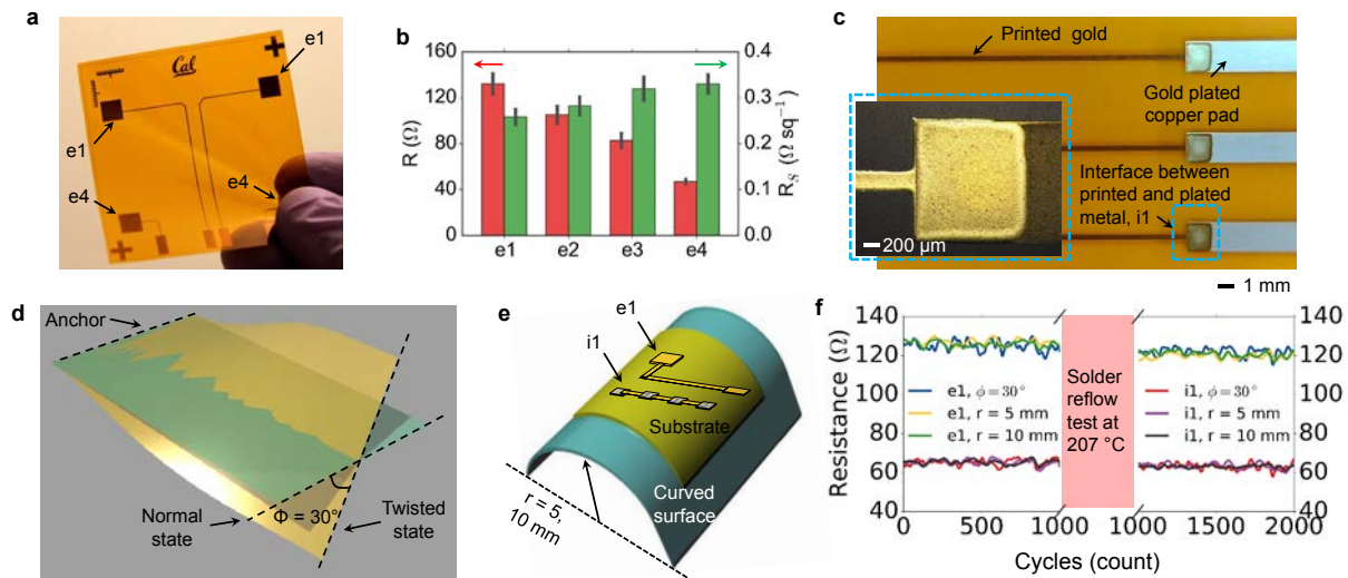
Figure 6.4. Electrical reproducibility and mechanical robustness testing of electrodes printed on Kapton ® PI and the interface between the printed gold and gold plated copper pad. (a) Photograph of printed electrodes of varying trace lengths. Four different trace lengths are used that are indicated by e1, e2, e3, and e4 (e1 and e4 are shown in the photograph as an example). (b) Line ( R ) and sheet resistance ( R_s ) of the electrodes (the bar chart data is collected from 10 electrodes of the same length, the error bars represent the standard deviation of the data). (c) Photograph of the interface between the printed gold and gold plated copper pad. The blue inset shows a micrograph of the interface. (d) Schematic illustration of the torsion testing setup. The printed device is anchored at two ends, the other two ends are twisted in opposing directions. Twist angle of \phi = 30^\circ is used for the twist cycles. (e) Schematic illustration of the bend testing setup. The printed devices are subjected to bending radii of 10 and 5 mm. (f) Mechanical robustness testing results. The resistance of a printed trace (e1) that is bent to 10 mm (green) and 5 mm (yellow) bending radius, and twisted to 30^\circ twist angle (blue). Similarly, the resistance of a line consisting of 6 printed/plated gold interfaces (i1) that is bent to 10 mm (black) and 5 mm (purple) bending radius, and twisted to 30^\circ twist angle (red). The first 1000 cycles of bending and twisting are done before the solder reflow test, then the printed devices are run through a solder reflow oven at 207^\circ\text{C} . The second 1000 cycles of bending and twisting are done after the solder reflow test. Noise in resistance measurements arose from instrumentation and wire-pad contact resistance variations.
