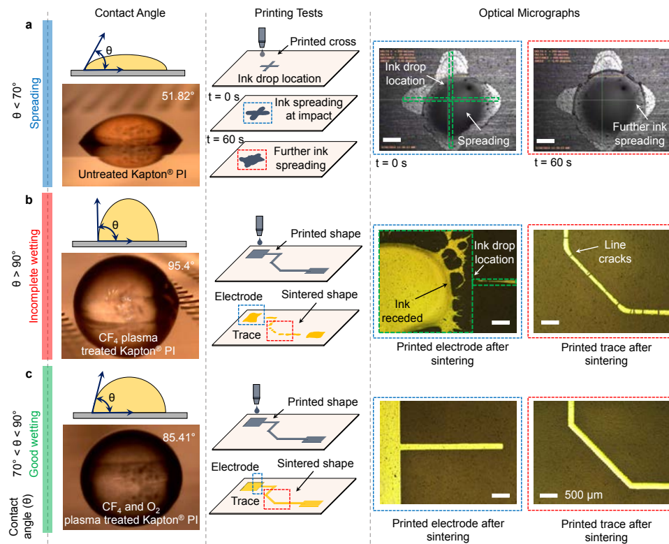
Figure 6.2. Surface energy optimizations for inkjet printing functional inks on Kapton ® PI substrate. Blue, red, and green colored rows show deionized (DI) water contact angle ( \theta ) schematically and obtained from a goniometer, inkjet printing trials, and optical micrographs of printed structures on Kapton ® PI surfaces that show ink spreading, incomplete wetting, and good wetting, respectively. The scale bars in the micrographs represent 500\ \mu\text{m} . (a) Printing tests on untreated Kapton ® PI that shows uncontrolled spreading of ink. The high surface energy of untreated Kapton ® PI generates a contact angle less than 70^\circ , which results in ink spreading as shown in the schematic of the “printed cross” and spreading of the ink (middle panel of a). The cross does not hold shape at impact, and the ink spreads further as shown by the micrograph that is taken 60 s after printing (right panel of a). (b) Printing tests on \text{CF}_4 plasma treated Kapton ® PI that shows incomplete wetting of printed ink. To reduce the surface energy, the surface was fluorinated with \text{CF}_4 plasma treatment, hence, the contact angle goes above 90^\circ . At this high contact angle, the printed ink recedes due to high cohesive forces within the ink, resulting in agglomeration of ink and dewetting clusters. The middle panel shows the schematic of a printed pad and an angled trace. Ink dewetting and line cracking are observed after sintering the gold nanoparticle ink. Micrographs of the pad and trace are shown in the right panel of b. Receding and agglomerating ink created discontinuities in the sintered shapes. (c) Printing tests on \text{CF}_4 and \text{O}_2 plasma treated Kapton ® PI that shows good wetting of printed ink. After the \text{O}_2 plasma treatment, the contact angle comes down to the printable range, 70^\circ < \theta < 90^\circ . In this case, high-quality printing is observed, as demonstrated by the micrographs of the printed pad and the angled trace in the right panel of c.
