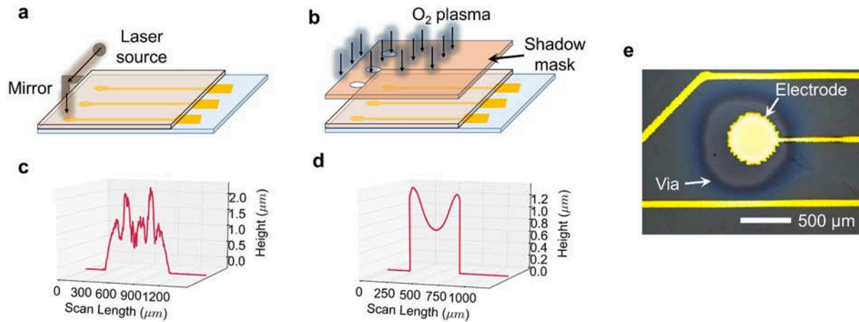
Figure 2.3. Methods for removing the dielectric layer (Cytos) from the electrodes. (a) Laser drilling to open via through the dielectric layer. (b) O_2 plasma etching using a shadow mask to selectively etch the dielectric layer. The surface profile of an electrode after (c) laser drilling and (d) plasma etching. (e) Micrograph of an electrode after plasma etching - etched area encircled by a dark Cytos layer, which is clearly visible; also the exposed electrode is shown.
