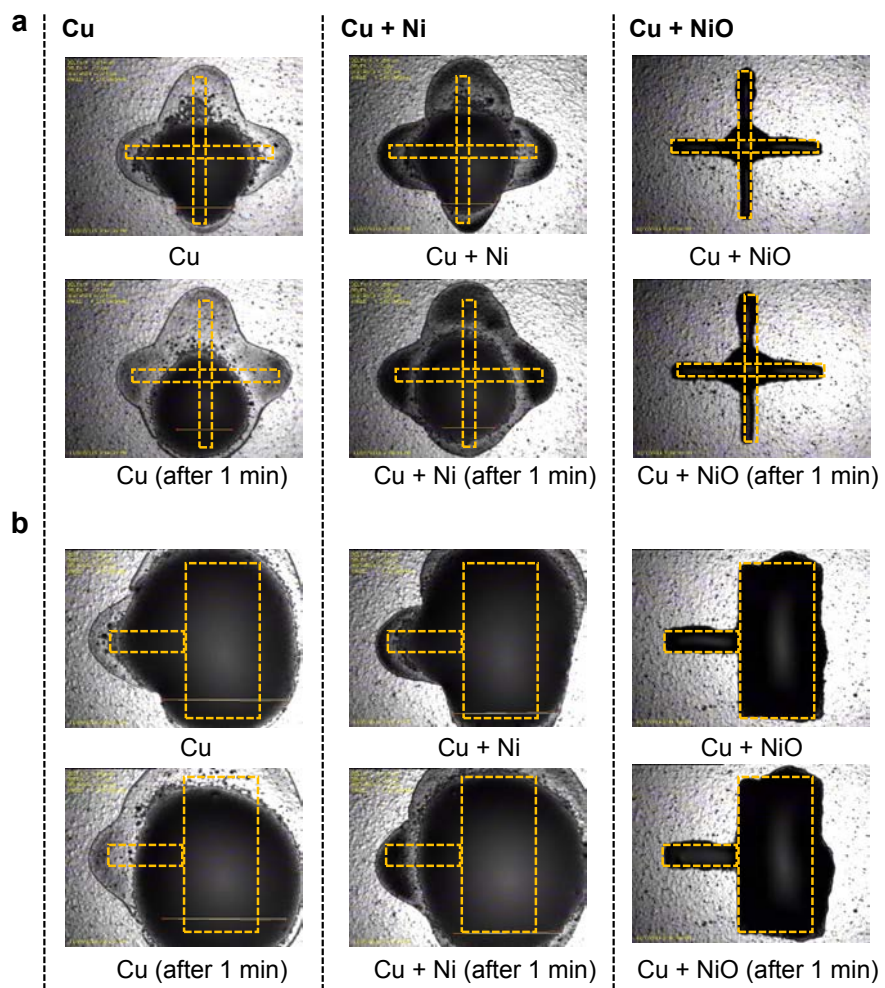
Figure 6.17. Nanoparticle ink wetting and spreading tests on different metallic surfaces. (a) 1\text{ mm} \times 1\text{ mm} printed cross and (b) 1\text{ mm} long and 500\ \mu\text{m} wide printed tab on different metallic surfaces. The yellow dotted lines show the intended feature shape. In both (a) and (b), the top panel shows feature definition right after printing, while the bottom panel shows feature definition 1 min after printing. The first column in (a) and (b) shows printing on plated copper. The second column in (a) and (b) shows ink spreading on a nickel on copper surface. After a bake at 190\ ^\circ\text{C} for 30 min in air, an oxide layer is formed on the top of the nickel surface which restricts ink spreading to the metal features. The third column shows printed ink on this oxide surface. The pattern fidelity of printed features on the oxidized surface demonstrates significant improvement over the bare nickel on copper surface.
