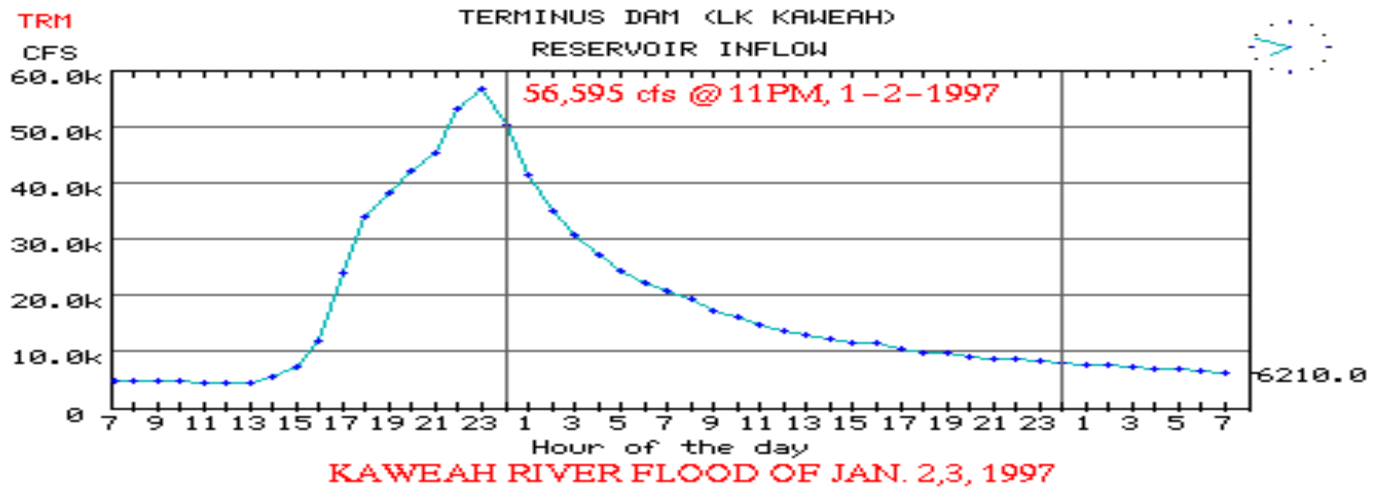
Figure 29. Discharge of the January 1997 flood.
