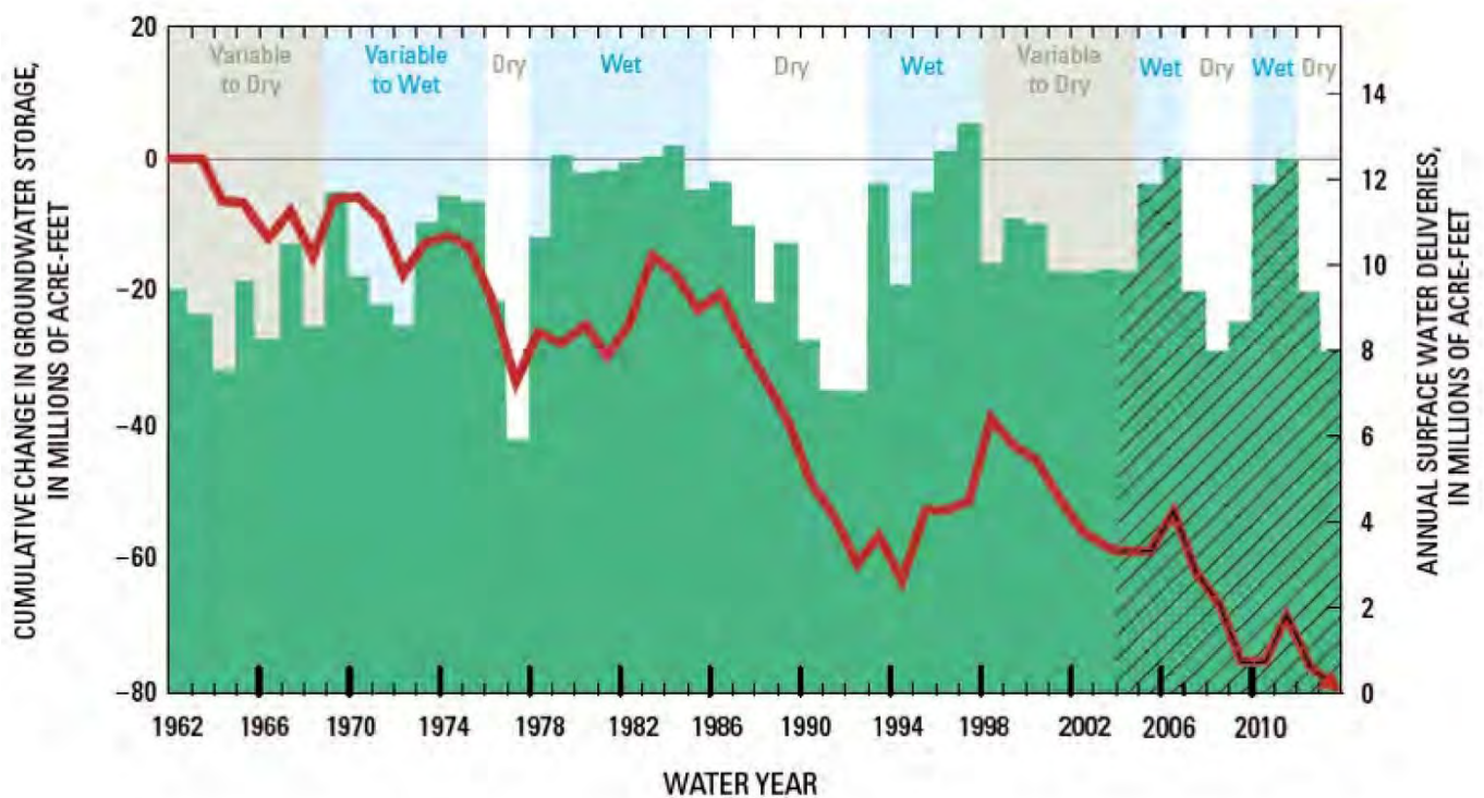
Figure 23. Amount of groundwater lost in past 52 years: 1962-2014. (million acre-feet)
