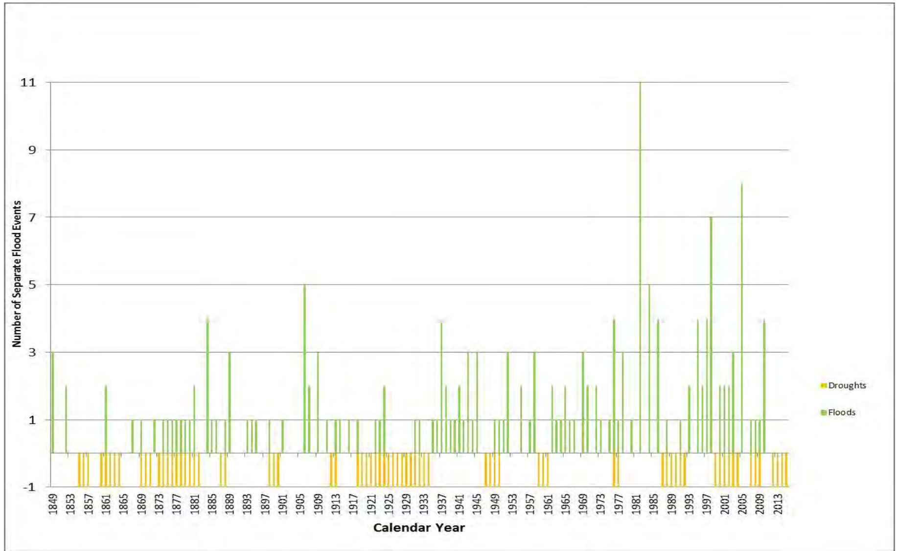
Figure 25. Known floods and multi-year droughts for past 167 years: 1849–2015.
