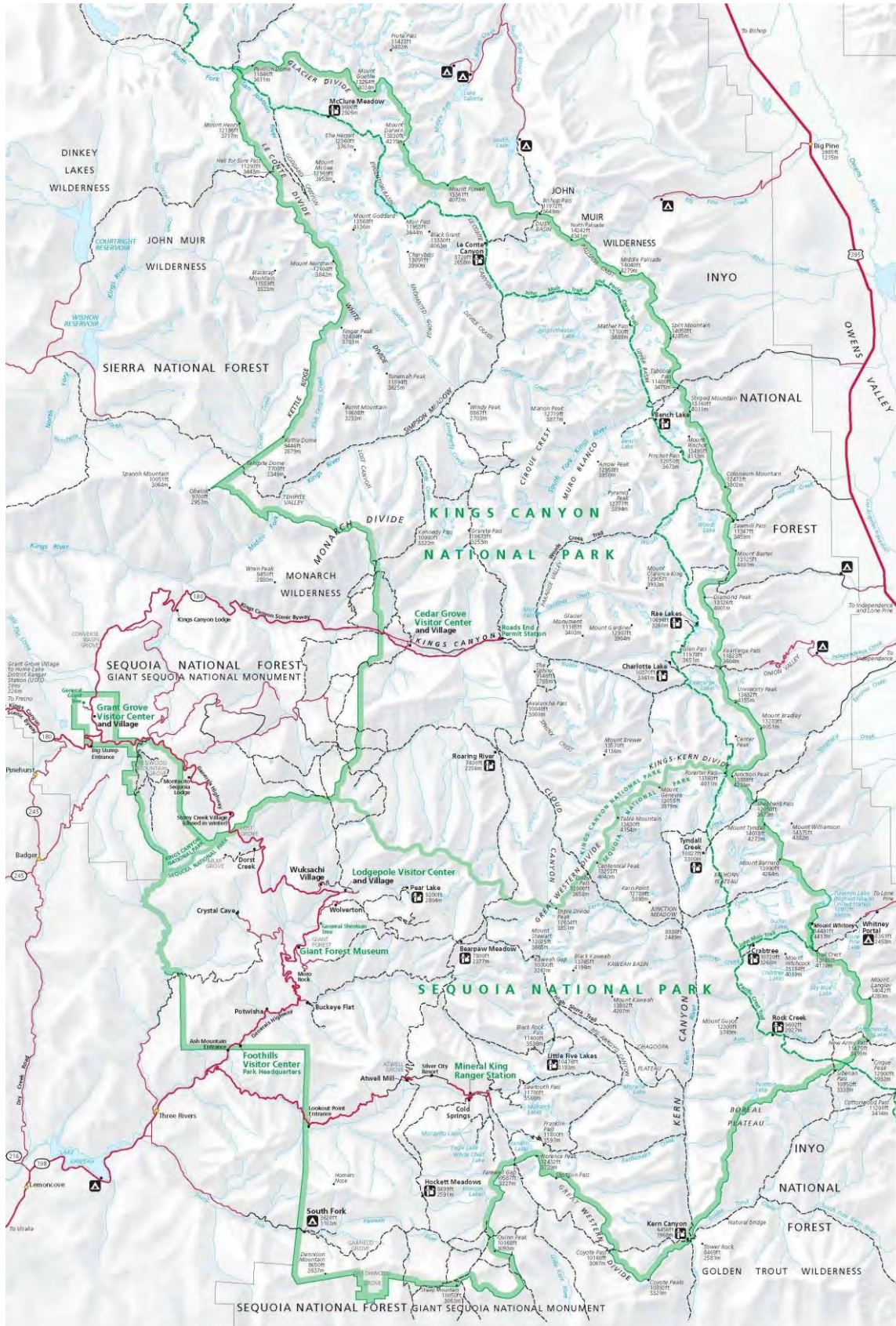
Figure 6. Map of Sequoia and Kings Canyon National Parks.
