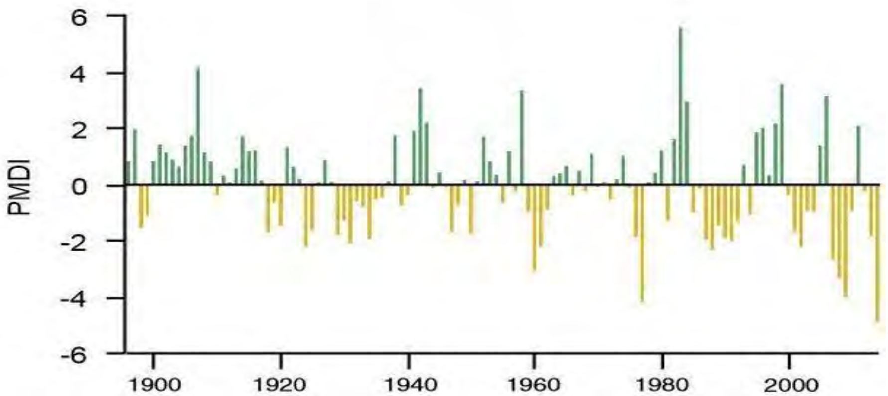
Figure 12. California drought severity (PMDI index) for past 119 years: 1896–2014.
