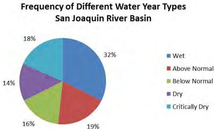
Figure 11. Frequency of different water year types in the San Joaquin River Basin (1901–2014).
