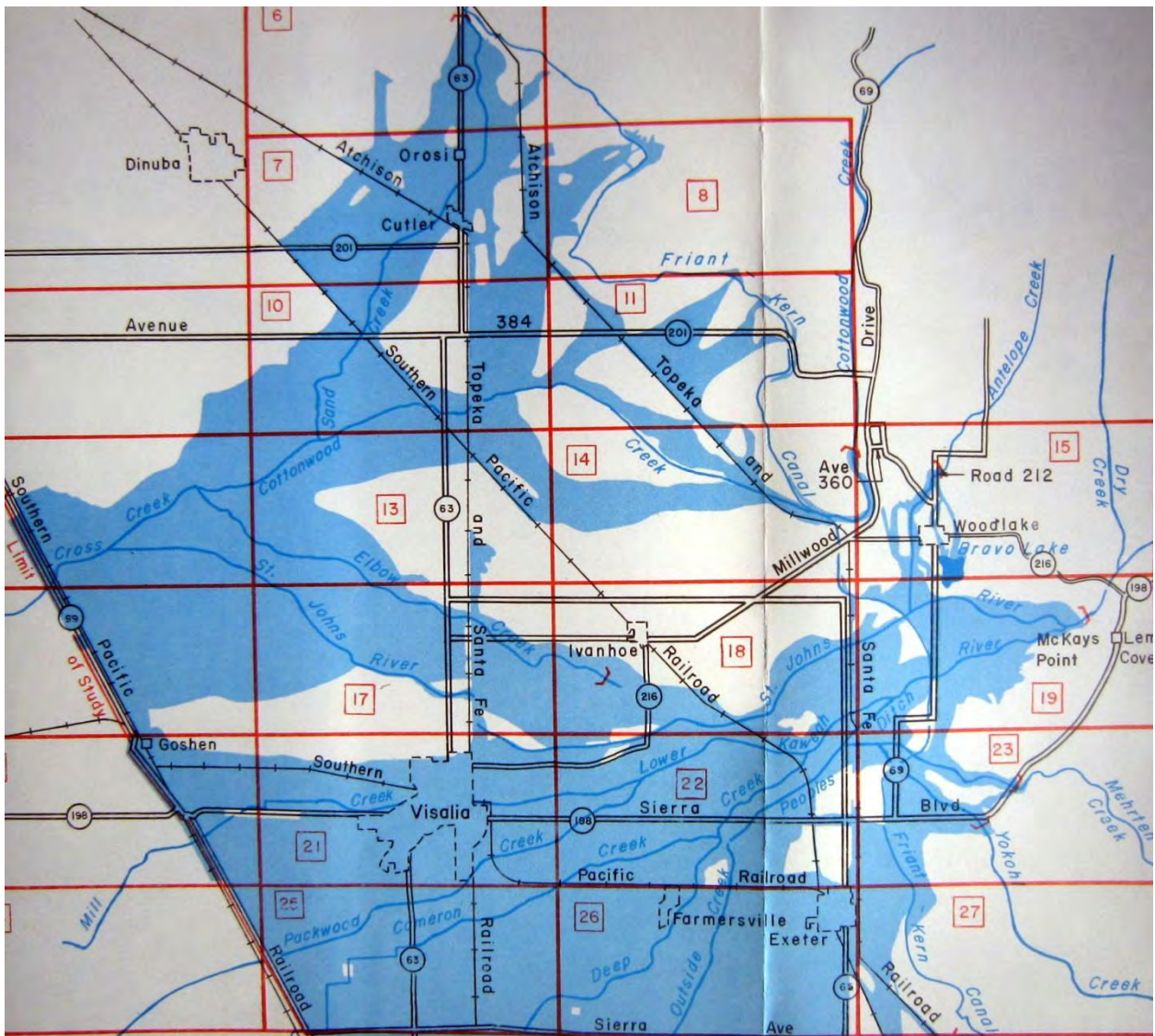
Figure 7. Standard project flood — Northwest Tulare County. Source: U.S. Army Corps of Engineers 53
