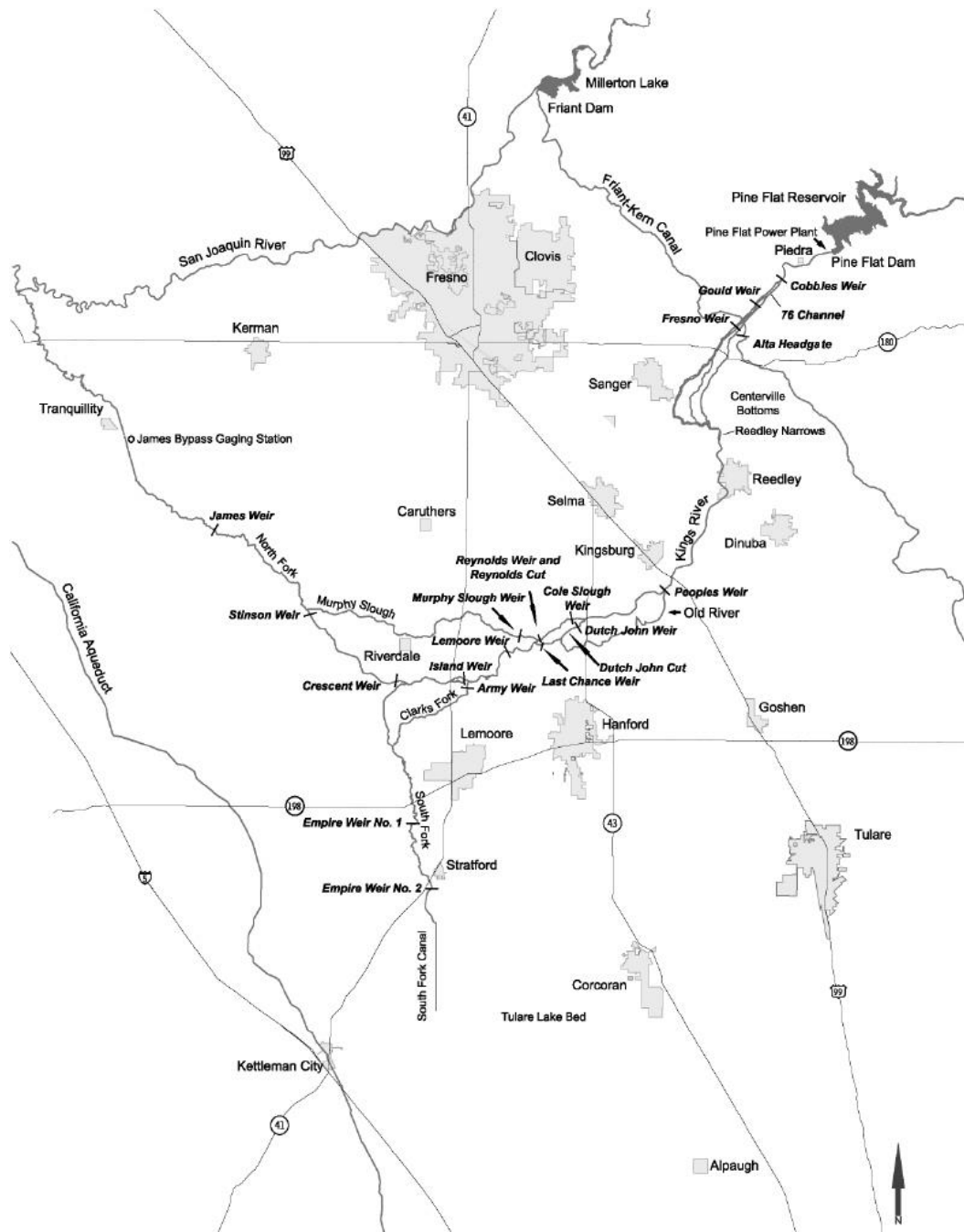
Figure 17. Map of Lower Kings River features. Source: Kings River Handbook
