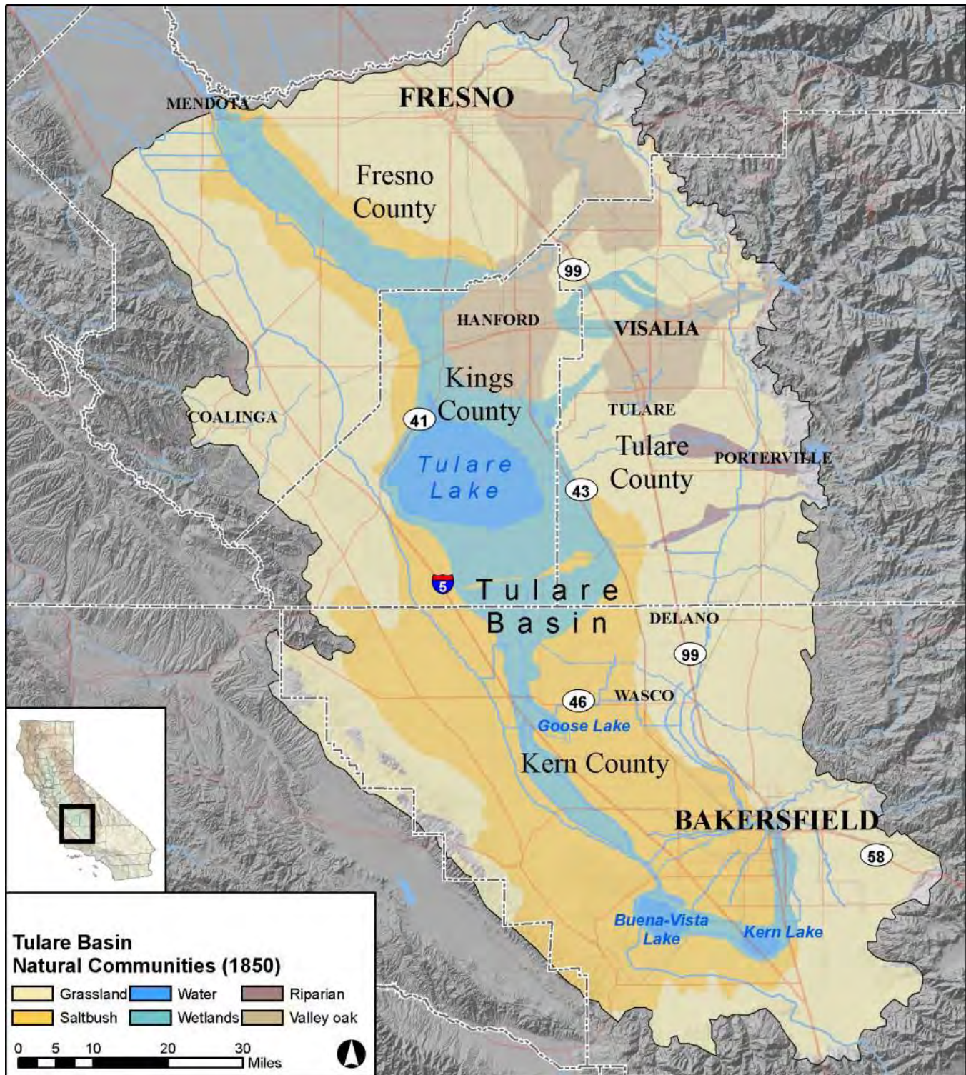
Figure 5. Map of Tulare Lake Basin natural communities. Source: Scott Phillips, CSU Stanislaus
