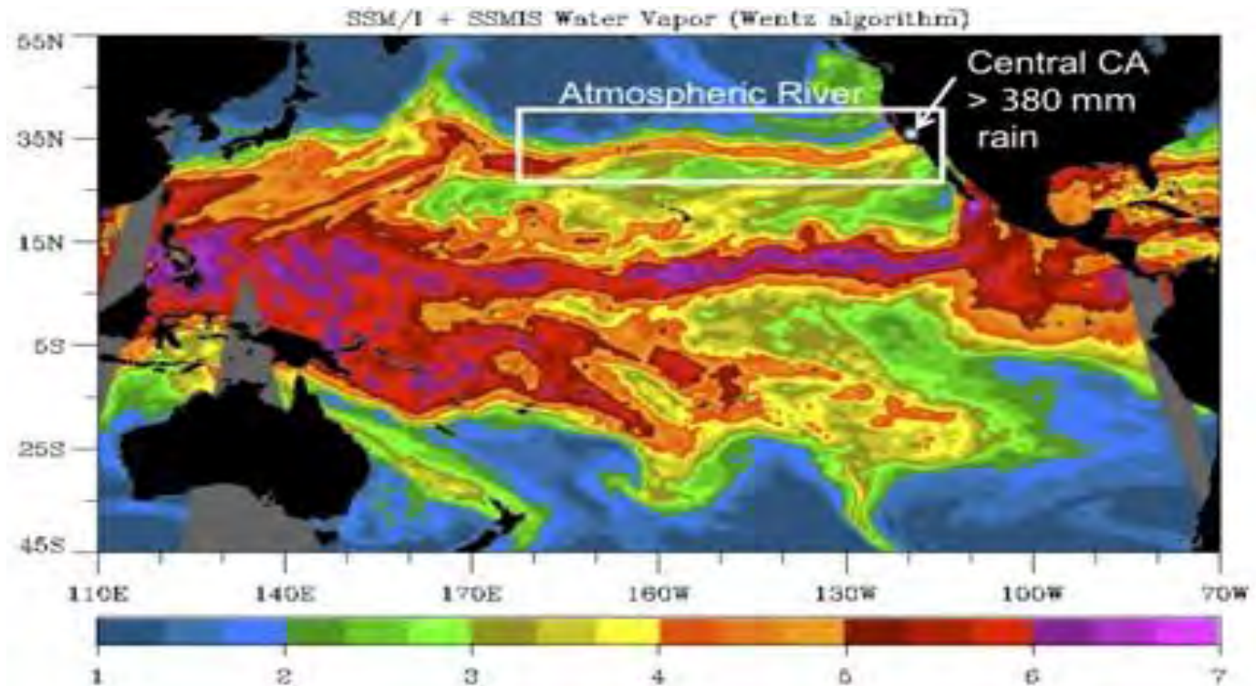
Figure 30. An atmospheric river channeling water vapor from the decaying Typhoon Melor across the Pacific Ocean to the Sierra on October 14, 2009.
