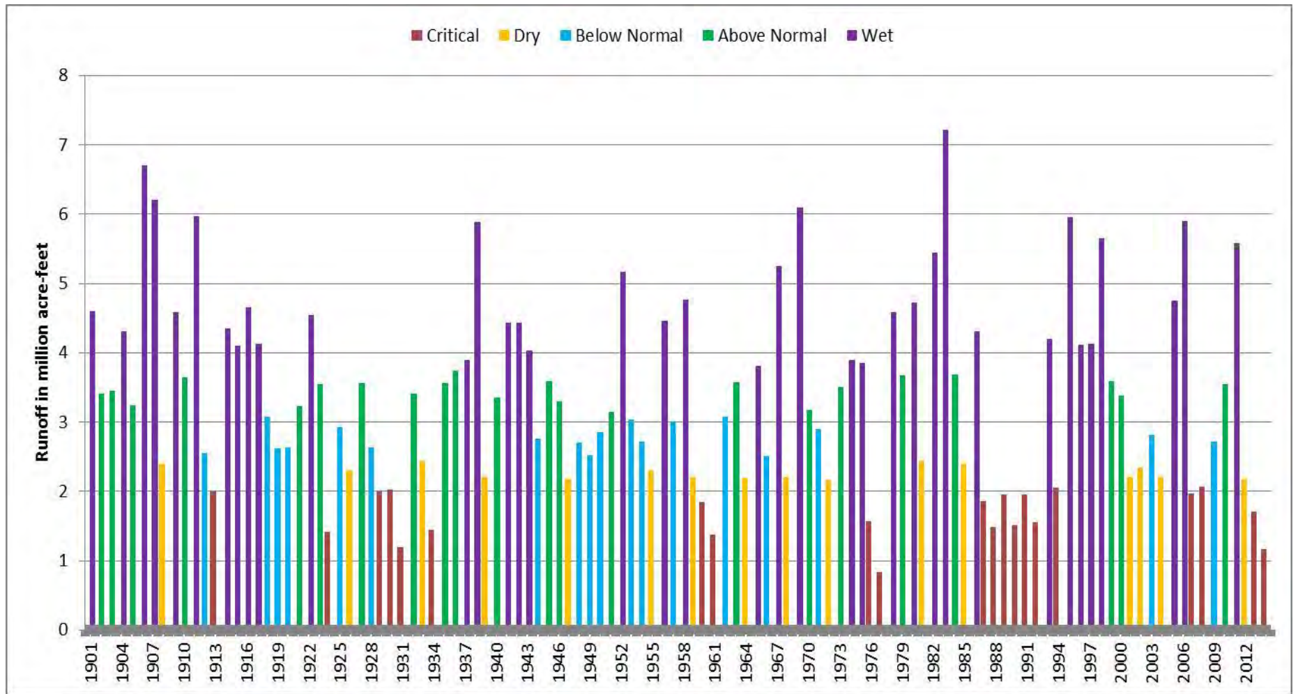
Figure 10. San Joaquin Valley Water Year Index for past 114 years: 1901–2014. Source: California Department of Water Resources
