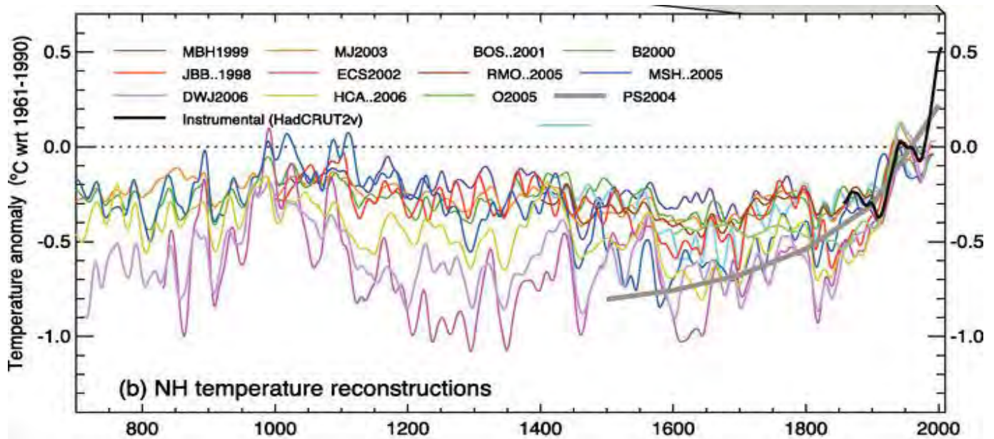
Figure 9. Northern Hemisphere temperature reconstructions for the last 1,300 years. Source: Intergovernmental Panel on Climate Change 2007 65
