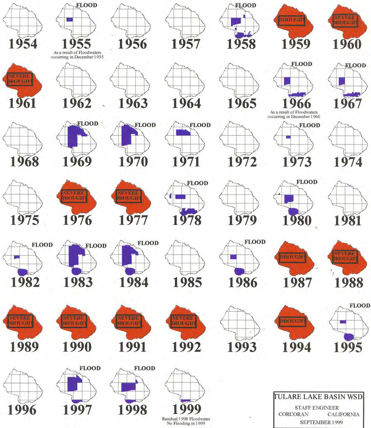
Figure 16. Portion of the Tulare Lakebed flooded each year 1954–99. Source: Tulare Lake Basin Water Storage District
