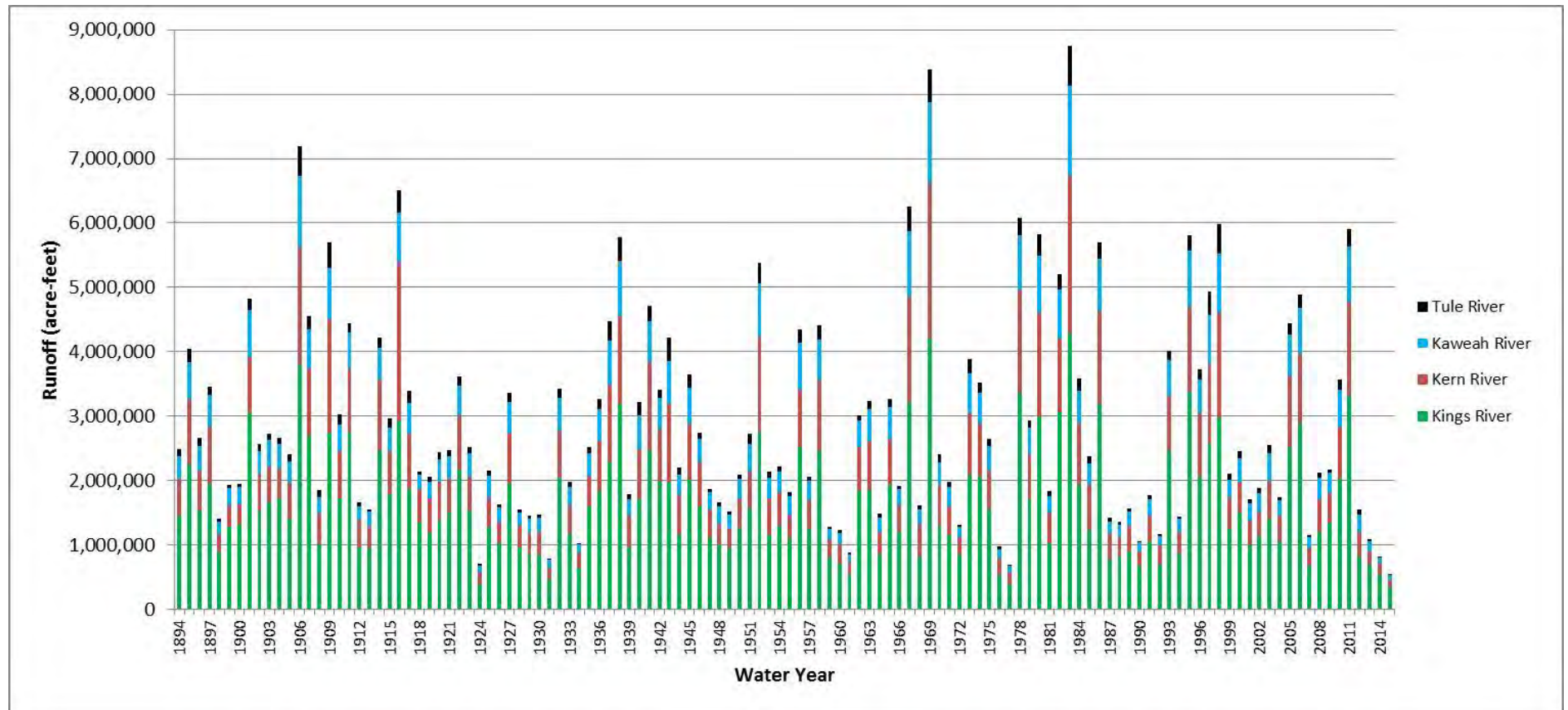
Figure 18. Variation in runoff over past 122 years: 1894–2015.
