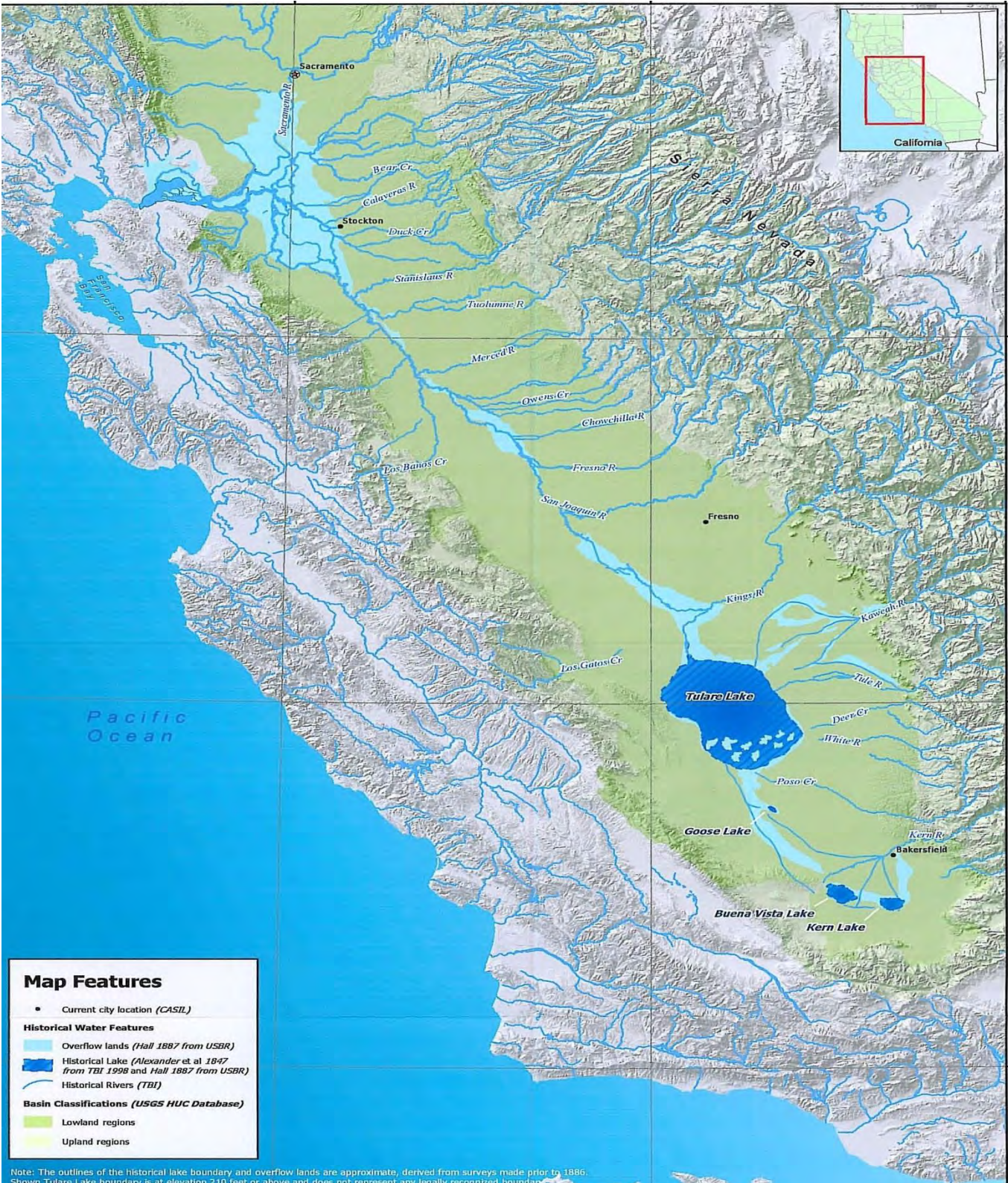
Figure 3. Map of San Joaquin Valley. Source: ECORP Consulting, report prepared for EPA. 3
