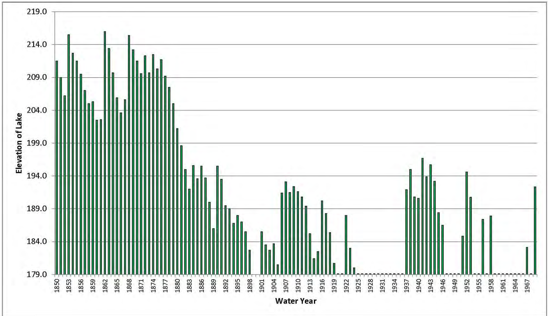
Figure 15. Elevation of water in the Tulare Lakebed for 120 years: 1850–1969. Source: Data from USBR which obtained it from USACE which compiled it from a variety of sources. 332
