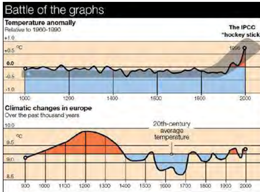
Figure 8. Comparison of two temperature reconstruction graphs.
