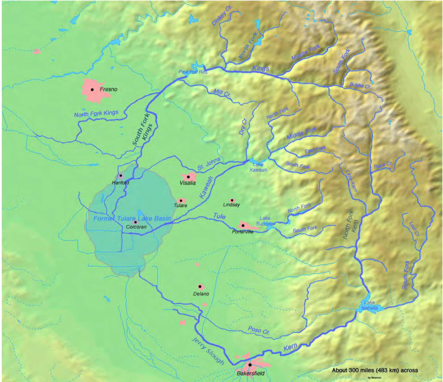
Figure 4. Map of Tulare Lake Basin. Source: Wikimedia Commons with corrections by Tony Caprio
