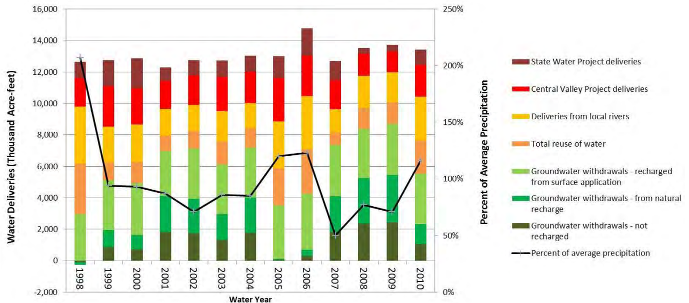
Figure 19. Sources of water — Tulare Lake Basin: 1998–2010.
