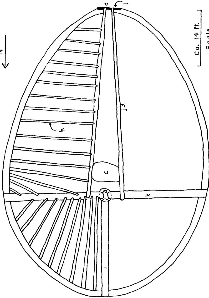
Top View
