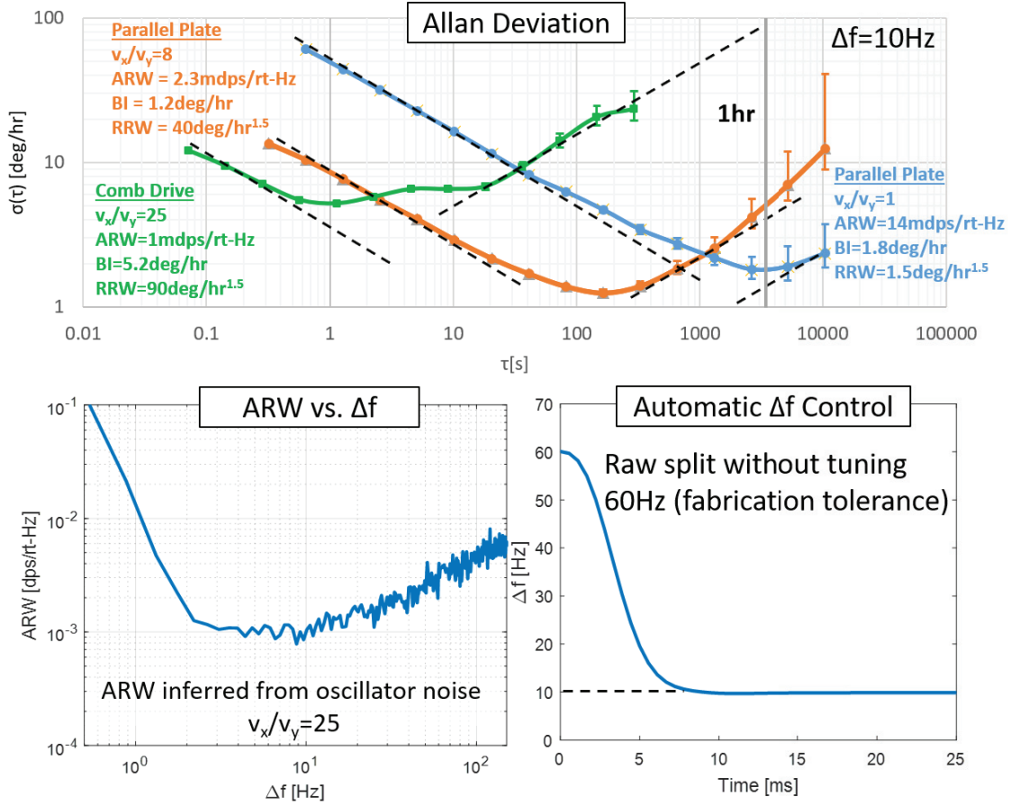
Figure 5.15. Allan deviation of the FM channel, ARW versus mode split, and automatic mode split tuning.
