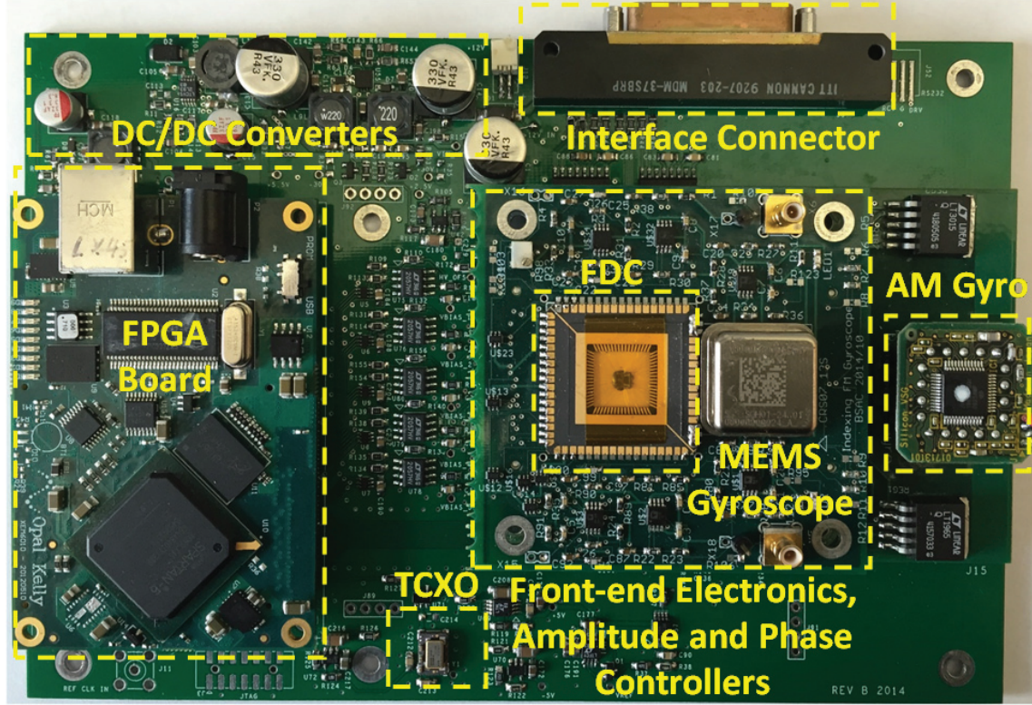
Figure 4.3. Board photo of the tested system.
