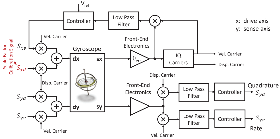
Figure 2.11. Simplified block diagram for force-feedback gyroscopes.
