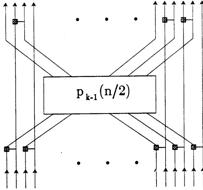
Fig.5.1 Recursive Construction of a P_k(n) Adder
