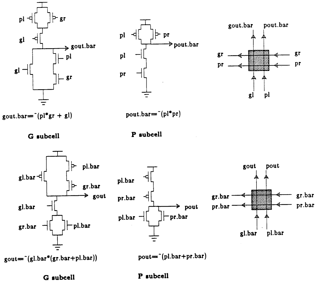
Fig.3.3 Black Cell Implementations in Static CMOS
