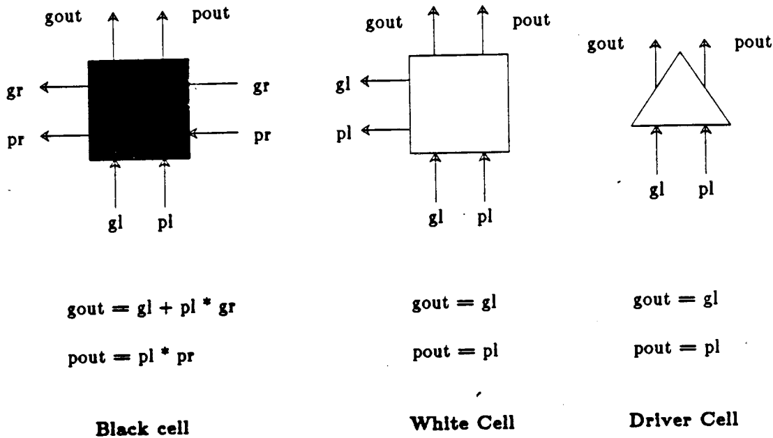
Fig.3.2 Three Basic Types of Adder Cells
