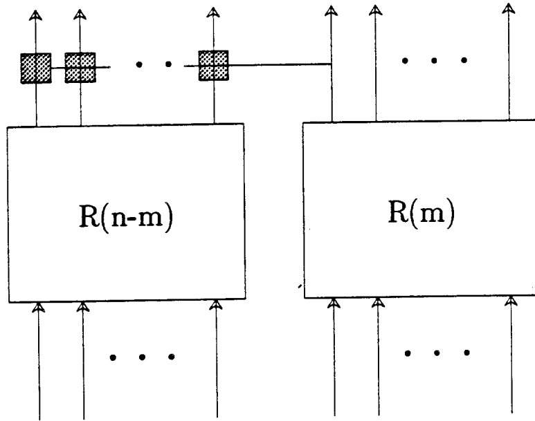
Fig.5.3 Recursive Construction of an R(n) Adder
