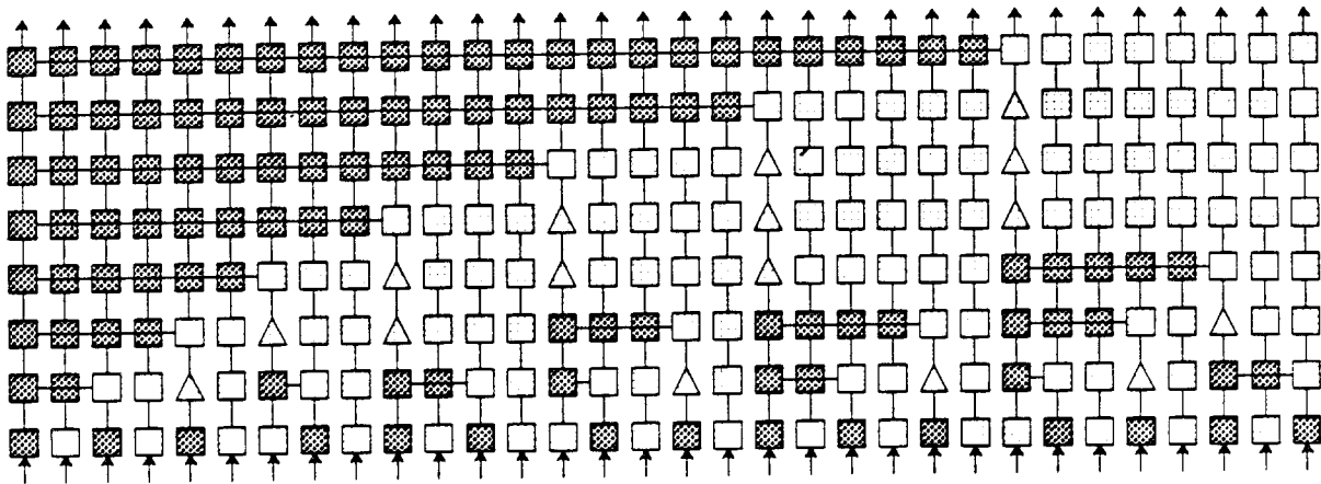
Fig.5.5 The Optimal 32-bit R(n) Adder
