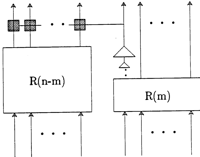
Fig.5.4 Drivers used in building an R(n) Adder
