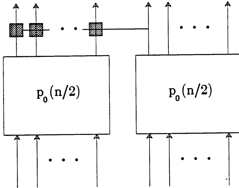
Fig.5.2 P_0(n) Adder Circuit
