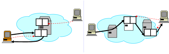
Figure 2: (a) An attacker learning the IP address of the i3 node that stores the victim’s public trigger (x, V) ( x and x' have the same prefix). (b) Possible solution: every i3 node responsible for public IDs won’t allow triggers pointing to end-hosts and won’t allow end-hosts to cache its IP address.
