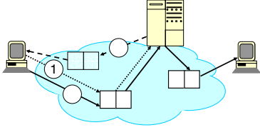
Figure 4: Slowing down a DoS attack on a public trigger.
