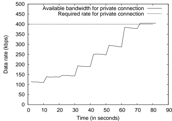
Figure 10: Reaction to DoS attack
