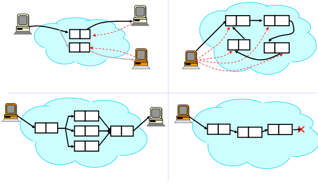
Figure 6: Security problems in i3 : (a) eavesdropping; (b) loop, (c) confluence, and (d) dead-end.
