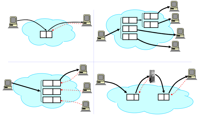
Figure 1: Basic communication primitives in i3 : (a) unicast, (b) multicast, (c) anycast, and (d) service composition.
